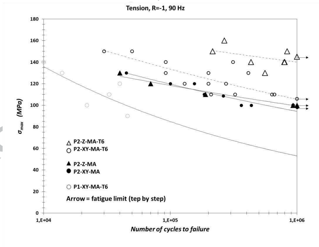
Figure 9: influence of the building direction, process parameters and T6 heat-treatment on the fatigue properties.
