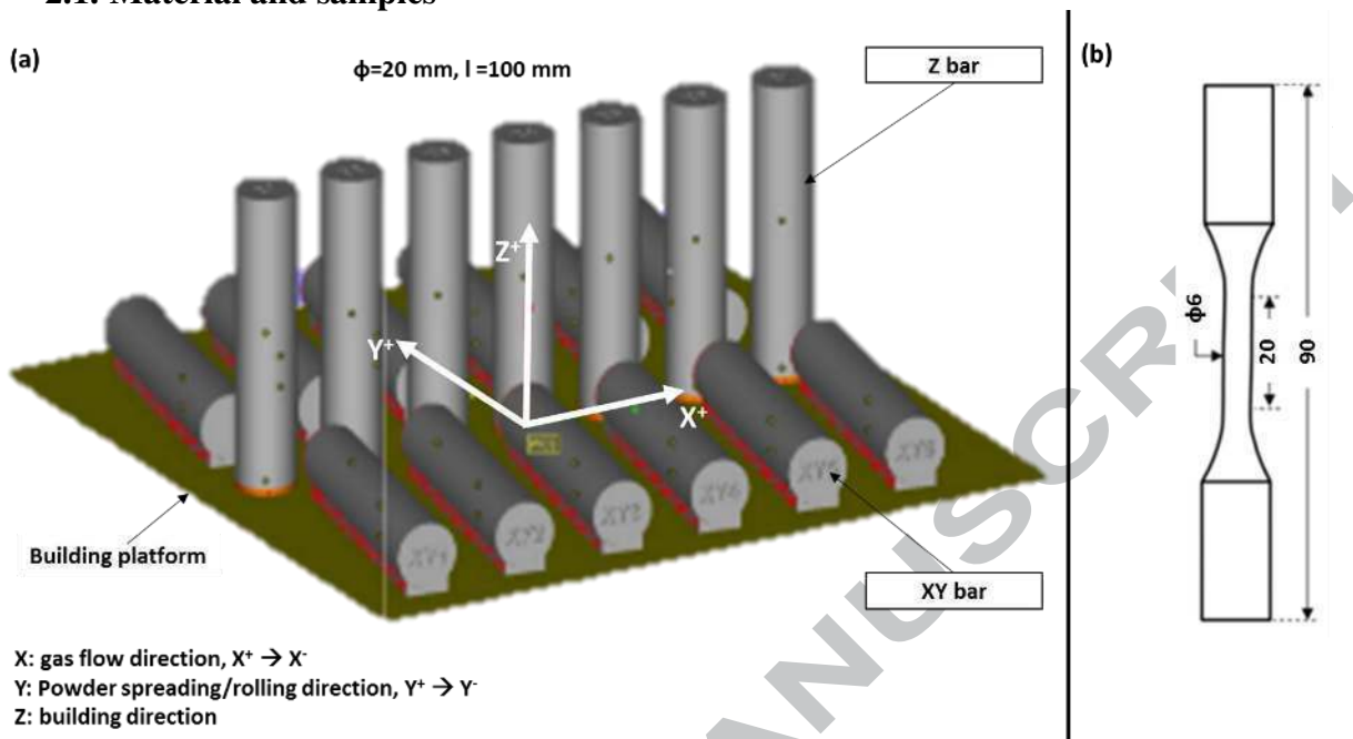
Figure 1: (a) Position and orientation on the building platform of bars from which fatigue specimens are machined, (b) Fatigue test specimen geometry, one bar corresponds to one specimen.
