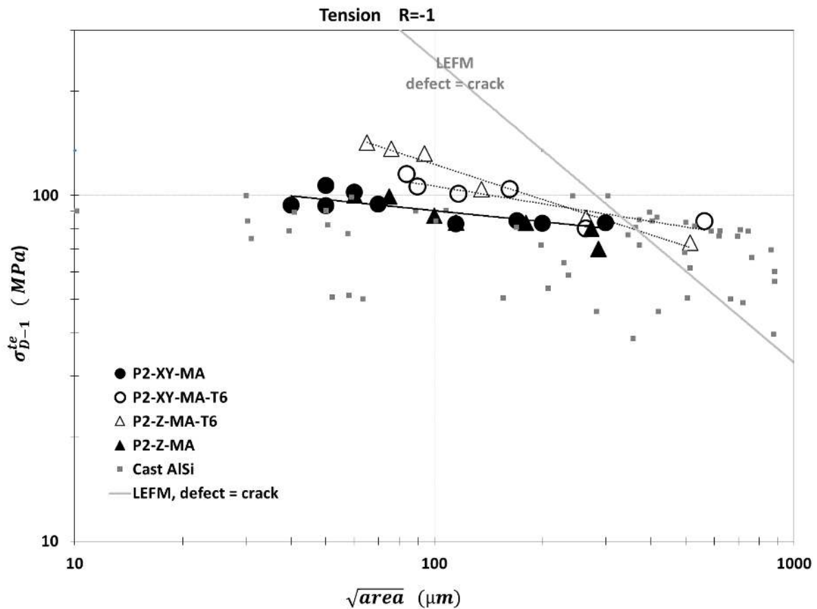
Figure 15: Fatigue limit as a function of defect size, comparison between additive manufacturing and conventional cast alloys [18, 24, 25, 27, 28, 42, 43].
