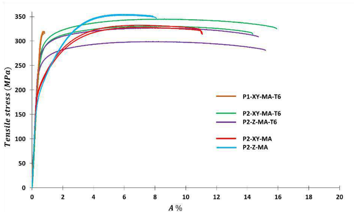
Figure 7: influence of the building direction and T6 heat treatment on the tensile properties of ALM AlSi10Mg alloy
