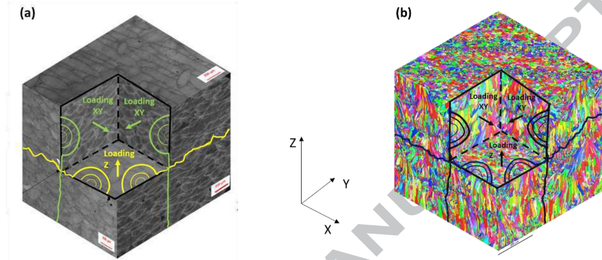
Figure 14: sketch explaining the difference observed on fatigue properties between XY and Z, (a) fatigue crack related to the melt-pools size (b) fatigue crack related to the grain size.
