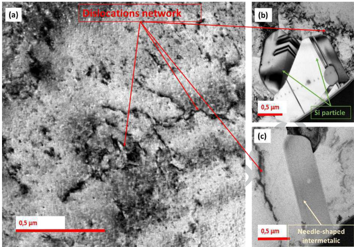
Figure 13: TEM bright-field image of a thin foil removed from bulk T6 and fatigue tested specimen. (a) A matrix with a high dislocation density (b) a twinned crystal of silicon containing no dislocations (c) an intermetallic that is also dislocation-lean.
