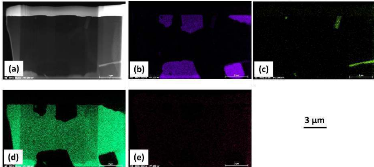
Figure 5: (a) SEI image without mapping. EDS mapping of chemical elements present in the alloy after T6. Distribution of (b) silicon (purple), (c) Iron (yellow), (d) aluminium (green), (e) Magnesium (orange).
