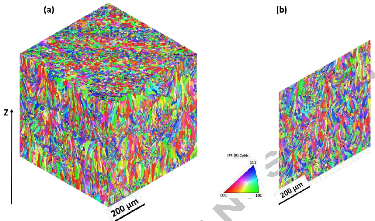
Figure 4: EBSD observations of the grain orientation, (a) 3D observation before T6 heat treatment, (b) XZ image after T6 heat treatment.
