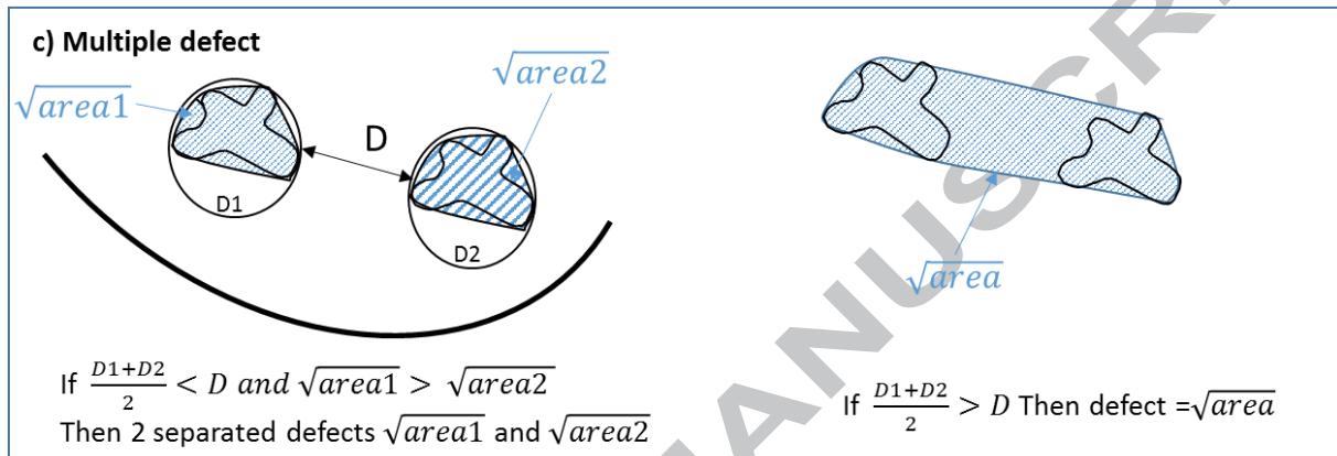
Figure 11: definition of the defect size depending on its location relative to the free surface, D1 and D2 are the diameters of a circles that encapsulates the corresponding defect.
