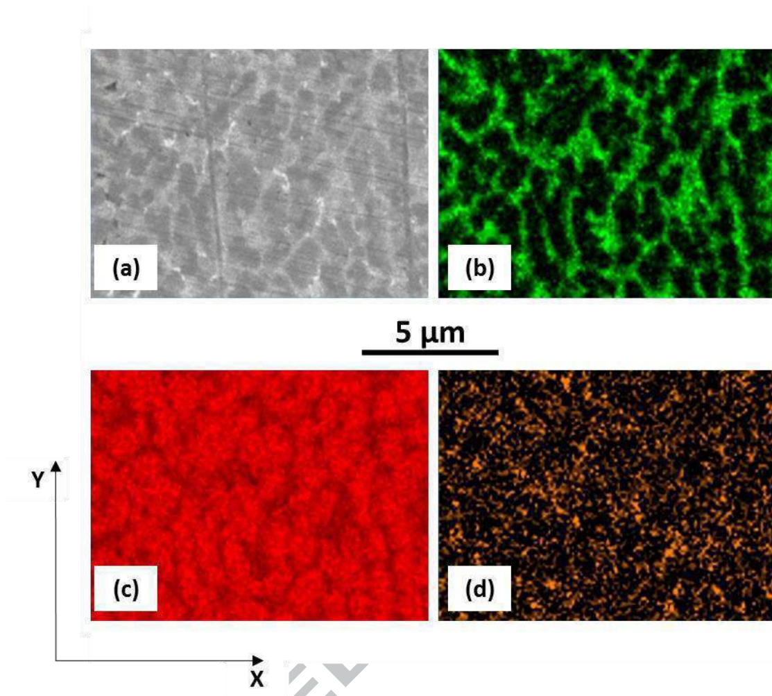
Figure 3: (a) SEI image without mapping. EDS chemical maps of elements present in the alloy without T6. Distribution of (b) silicon (green), (c) aluminium (red), (d) Magnesium (orange).
