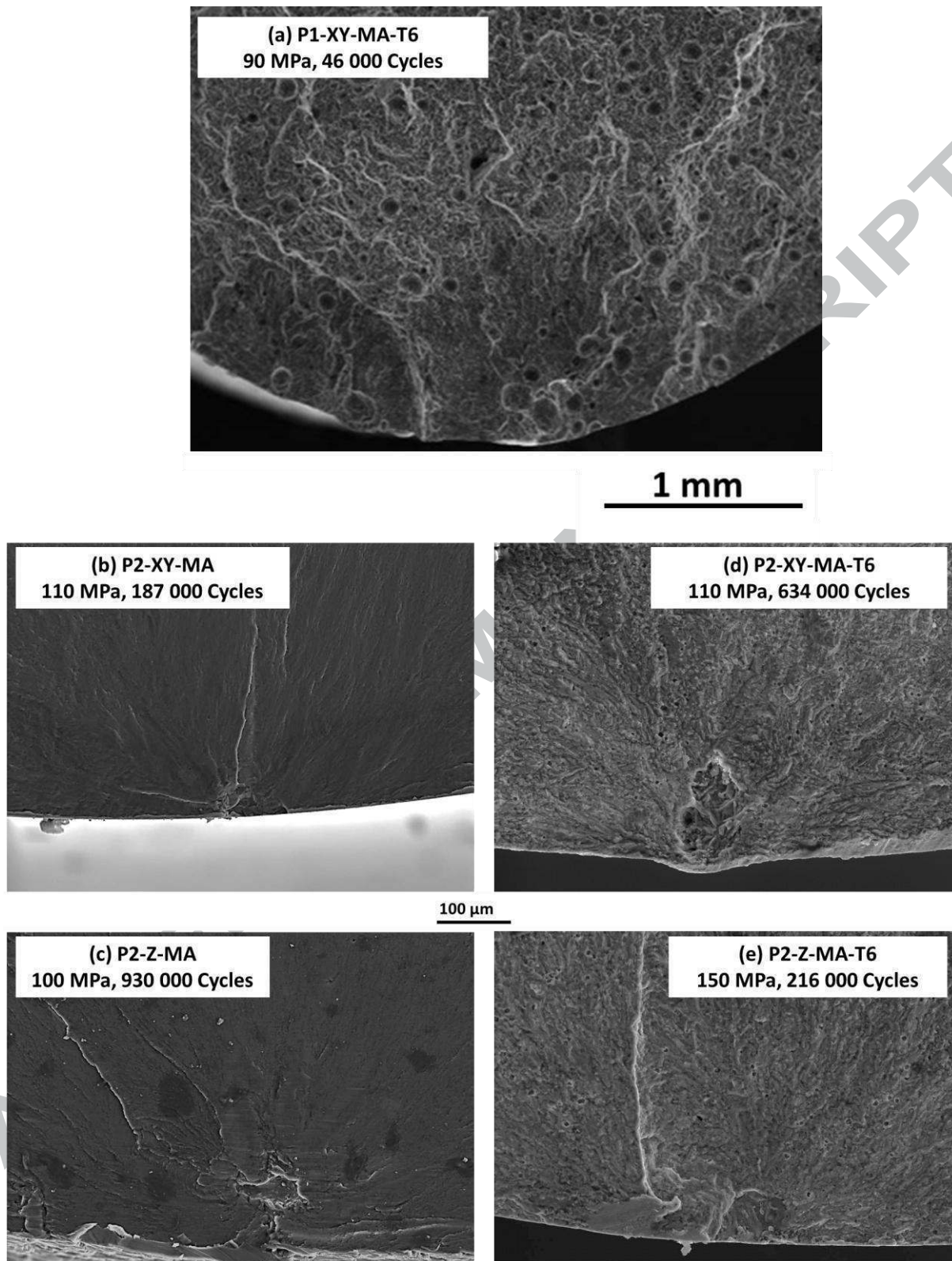
Figure 10: SEI images of fracture surfaces and initiation sites. (a) P1-XY-MA-T6, (b) P2-XY-MA, (c) P2-Z-MA, (d) P2-XY-MA-T6 and (e) P2-Z-MA-T6
