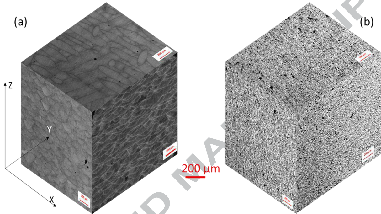
Figure 2: optical dark field microscopy 3D reconstructions of the microstructure after surface polishing, without etching, (a) without heat treatment (b) after T6
