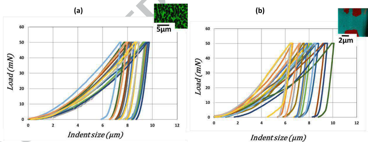
Figure 8: micro hardness characterization of P2 material. Highlighting of the results scatter via the load and discharge curves. (a) no T6, (b) after T6
