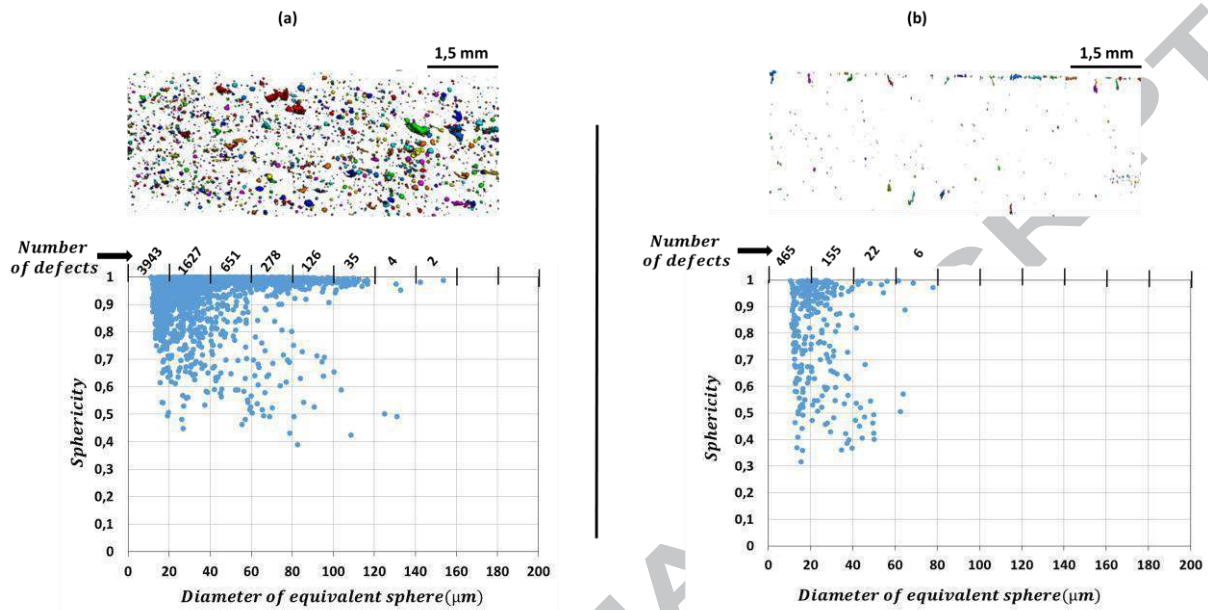
Figure 6: defect characterization of P1 and P2 production. The top images give the special repartition of defects in observed zone while bottom show the number of defect and sphericity distribution related to the equivalent diameter (a) P1 production, (b) P2 production.
