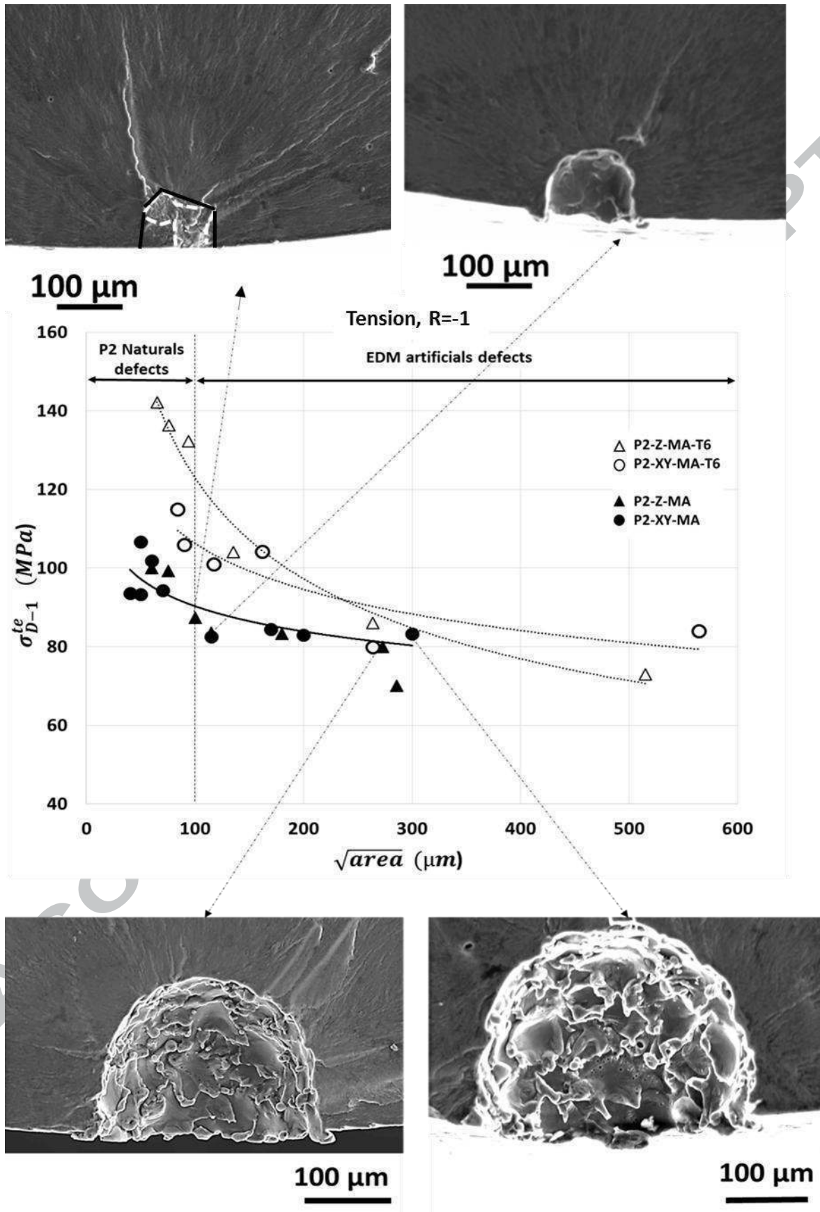
Figure 12: Kitagawa type diagram showing the impact of defect size on the fatigue limit after or not heat treatment for two building direction XY and Z
