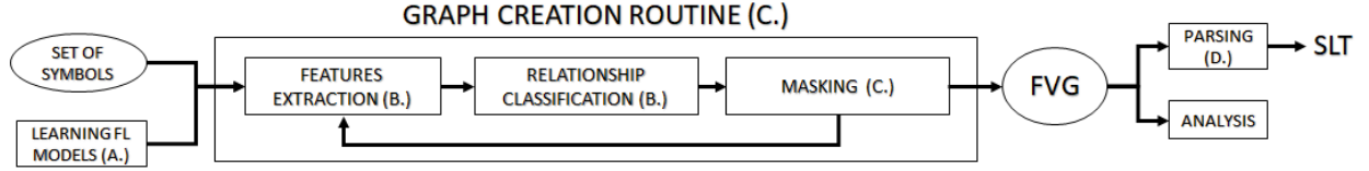
Fig. 2: Overview of our system. Using a set of segmented and classified symbols and a set of FL models learned as the input, an FVG is created from the models and additional features. The FVG is parsed to obtain the SLT.
