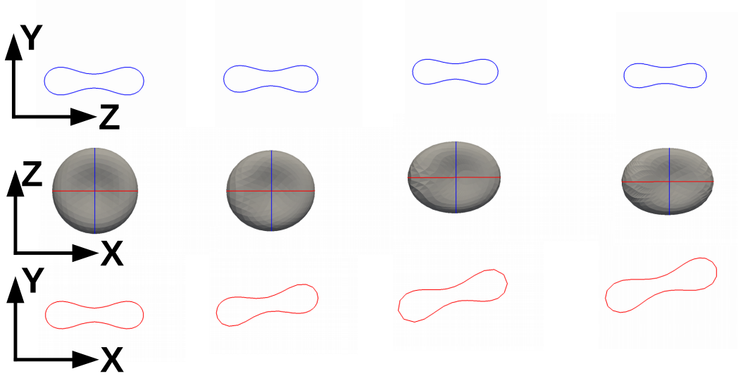
Fig. 6. Dynamics of lift of a biconcave vesicle ( v = 0.635 ; Ca = 0.375 ): Snapshots in the Z - Y plane (top row), X - Z plane (middle row) and X - Y plane (bottom row), for different dimensionless times (from left to right \dot{\gamma}t = 0; 2; 5; 10 ).
