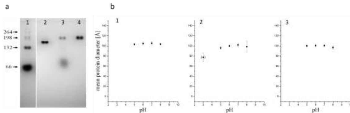
Figure 2. Multimeric size of the NpDps4, NpDps5, and EcDps analysed by non-denaturing PAGE and Dynamic light scattering (DLS). Non-denaturing PAGE (a) shows theoretical molecular masses of putative dodecamers were 262 kDa for NpDps4 (a1), 210 kDa for NpDps5 (a2), and 236 kDa (a3) for EcDps. Additionally, the different native forms of bovine serum albumin (BSA) were used for estimating the approximate molecular masses. The pH of the gel was 8.45 and the pH of the running buffer was 8.0. Dynamic light scattering (b) shows the hydrodynamic diameters of NpDps4 (b1), NpDps5 (b2) and EcDps (b3) proteins at different pH. All protein species are displayed as a mean of the average hydrodynamic diameter from each experimental series in (Å) at pH 3.0, 5.0, 6.0, 7.0 and 8.0. Particles with a lower peak occurrence than 1% (number related) are not shown, whereas particles with occurrence between 1% and 10% are shown in brackets. Standard error of the mean particle diameters is given as error bars.
