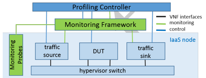
Fig. 2. The measurement setup used for profiling the VNFs.
