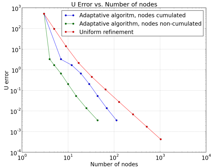
Figure 4: energy norm error in energy like potential with respect to number of nodes.
