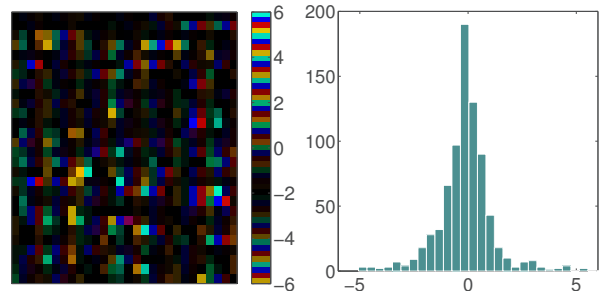
Fig. 1. MNIST one-vs-all experiment: Example of the MMSE estimator of a weight vectors \beta learned by SPA for the 2-vs-all binary classifier (left) and its associated histogram (right).
