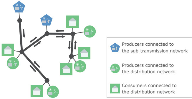
Fig. 2. Energy flow in future electrical networks
