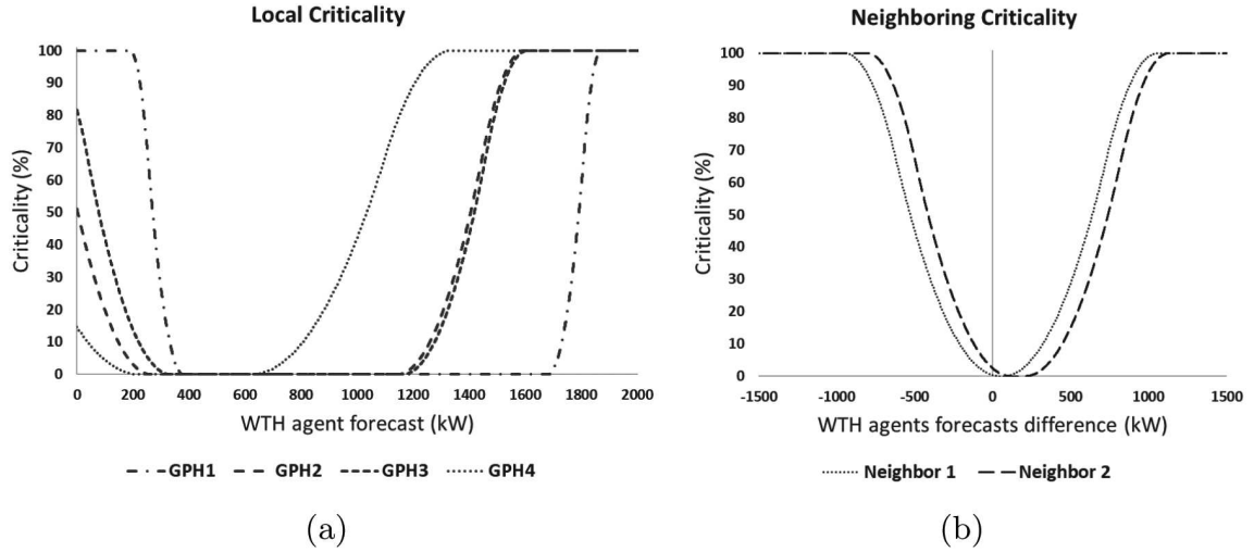
Fig. 4. Criticality decomposition: local (a) and neighboring (b)
