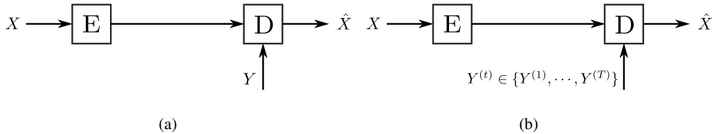
Fig. 1: (a) Slepian-Wolf source coding, (b) Source coding with several possible side informations at the decoder
