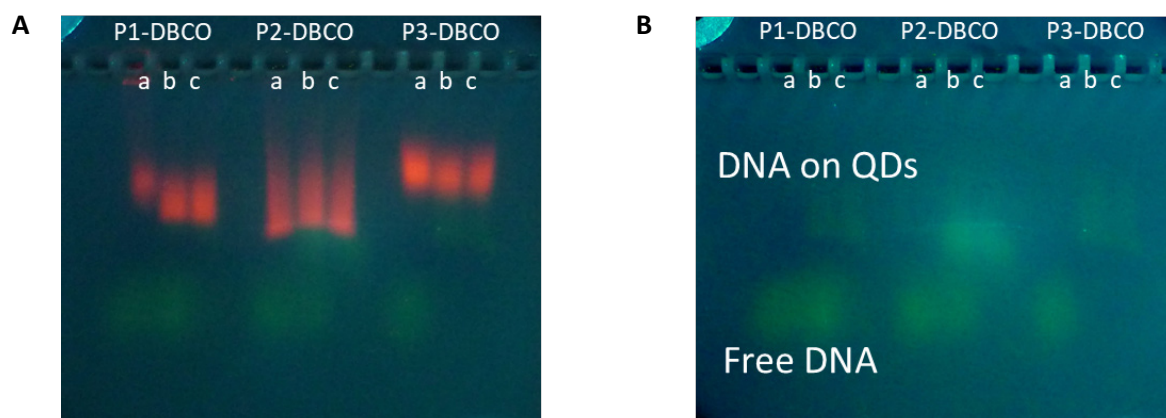
Figure S15: Image of 1% Agarose gel in 1X TBE buffer stained with SybrGreen taken with a camera on the home-made setup. All QD@P-DBCO are loaded at the same concentration with the same reaction conditions. Labels correspond to conditions listed in Table SI 6. (A) Imaging with bandpass emission filter enables visualization of both QD and DNA fluorescence. (B) Imaging with shortpass + bandpass filter exhibits only DNA fluorescence.
