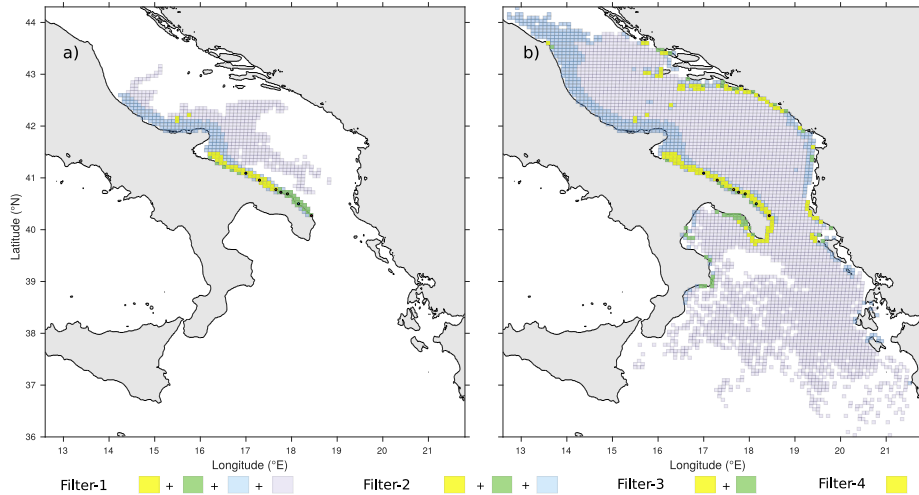
Figure 3: Spatial scales of dispersion as given by the characterization of larval sources by successive filtering procedure for D. sargus (panel a) and D. vulgaris (panel b).
