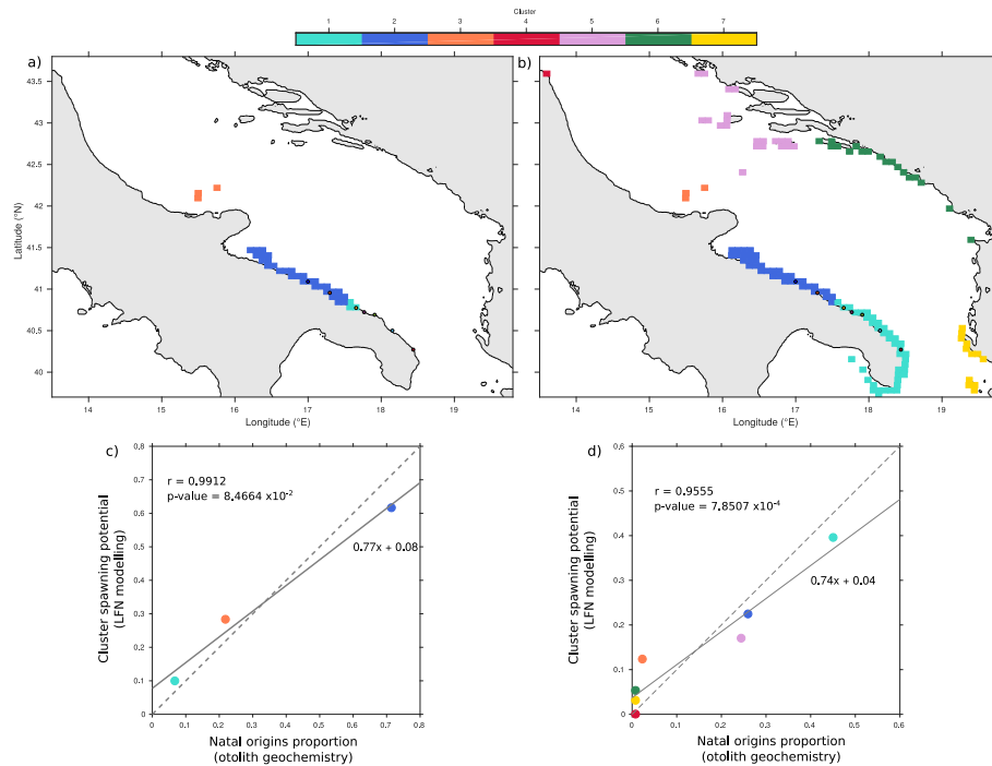
Figure 5: Spawning areas geographically-delimited thanks to criteria delimited thanks to criteria defined in section 2.5 and characterization of their relative contributions to the total pool of larvae settled in the Apulian coast. Clusters of the most constrained larval sources (panels a, b) and correlations between simulated larval contributions and observed natal origin proportions (panels c, d) for D. sargus (panels a, c) and D. vulgaris (panels b, d).
