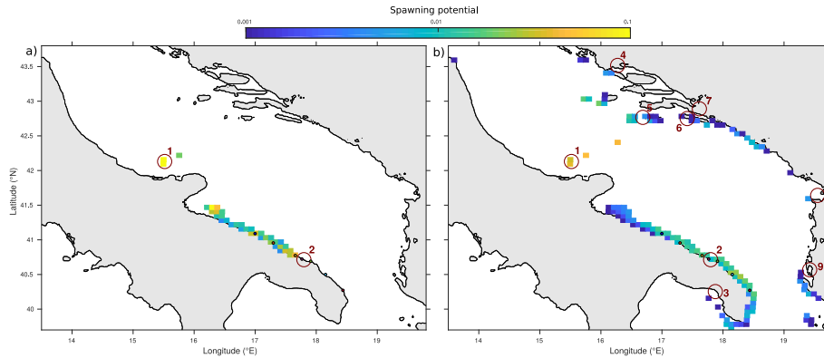
Figure 4: Quantitative patterns of connectivity for D. sargus (panel a) and for D. vulgaris (panel b): maps of the most constrained larval sources (after applying the superposition of the four filters), along with their associated probabilities (the probability of that node to supply larvae to the surveyed stretch of Apulian coastline) which are integrated here as the larval source’s spawning potential. Red circles represent the current Marine Protected Areas (MPAs) which have connection with the sampled locations: (1) Tremiti islands, (2) Torre Guaceto, (3) Porto Cesaro, (4) Pantana, (5) Lastovo archipelago, (6) Mljet, (7) Mali Ston Bay, (8) Lumi Buna-Velipoje and (9) Karaburun-Sazani Island (see SI B-7).
