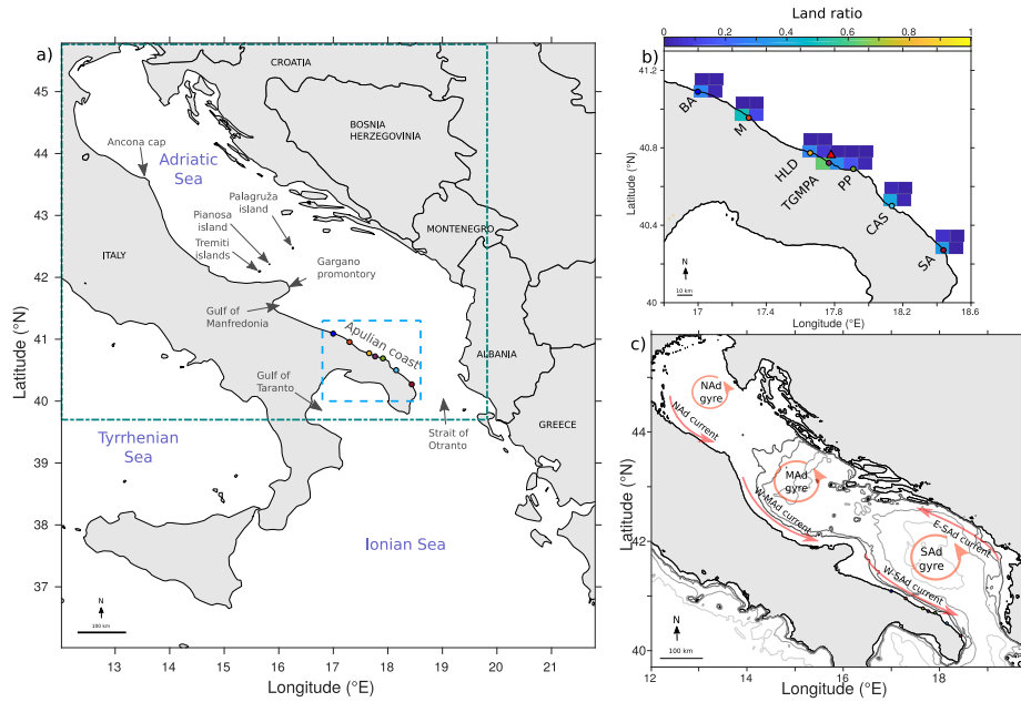
Figure 2: Geographical location, topography and schematic circulation of the study area. Panel a) displays the network domain (36 °- 46 °N, 12 °E - 22 °E ). Panel b) discloses a zoom over the Apulian coast and indicates the seven locations (colored dots) named, from north to south: Bari (BA), Monopoli (M), Hotel La Darsena (HLD), Torre Guaceto Marine Protected Area (TGMMPA), Punta Penna (PP), Casalabate (CAS) and San Andrea (SA). Location nodes , associated with each sampling location, are colored according to their land ratio (see SI A-1.1). The red triangle corresponds to the barycenter of all location nodes centers. Panel c) presents a schematized view of the mean surface circulation of the Adriatic Sea (red arrows). The system is dominated by the Western South Adriatic (W-SAd) current, the Eastern South Adriatic (E-SAd) current, the Western Middle Adriatic (W-MAd) current, the Northern Adriatic (NAd) current, the South Adriatic (SAd) gyre, the Middle Adriatic (MAd) gyre and the North Adriatic (NAd) gyre (adapted from Artegiani et al., 1997b; Millot and Taupier-Letage, 2005). The thin grey lines in panel c) corresponds to isobaths 80 m, 100 m, 200 m and 1000 m, respectively.
