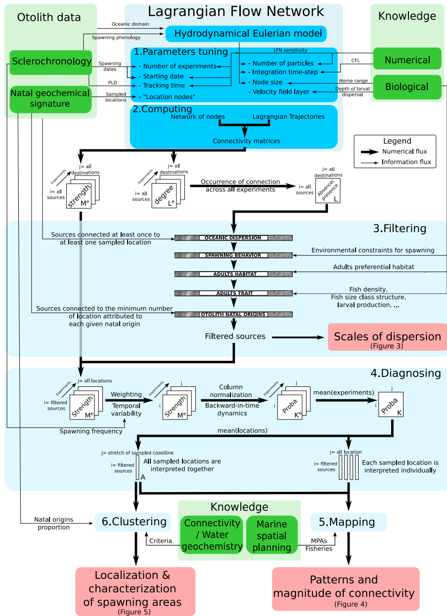
Figure 1: Schematic representation of our integrative framework which combines Lagrangian modelling and expert knowledge (including otolith analyses) in order (i) to investigate the scales of dispersion, (ii) to determine the patterns and magnitude of connectivity and (iii) to locate and characterize spawning areas for conservation purposes. Our framework is structured according to the color code: blue annotations refer to the numerical methodologies, green annotations symbolize expert knowledge (from existing bibliography) and red boxes highlight the key results. PLD stands for Pelagic Larval Duration and CFL for Courant-Friedrichs-Lewy (see section 2.2) for a definition of all the terms used).
