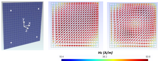
Fig 1: Iron sheet mesh and inversion test configuration (dimensions: 1m^2 , number of elements: 440, number of unknowns: 760, thickness: 2 mm, 4 tri-axis sensors at 5 cm from the sheet). Left: mesh and sensors location. Middle: reference H_c . Right: Identified H_c . The same range is provided for both H_c .
