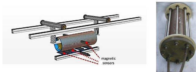
Fig 2: Plans of the experimental set up (left), pressurized cylinder (right).
