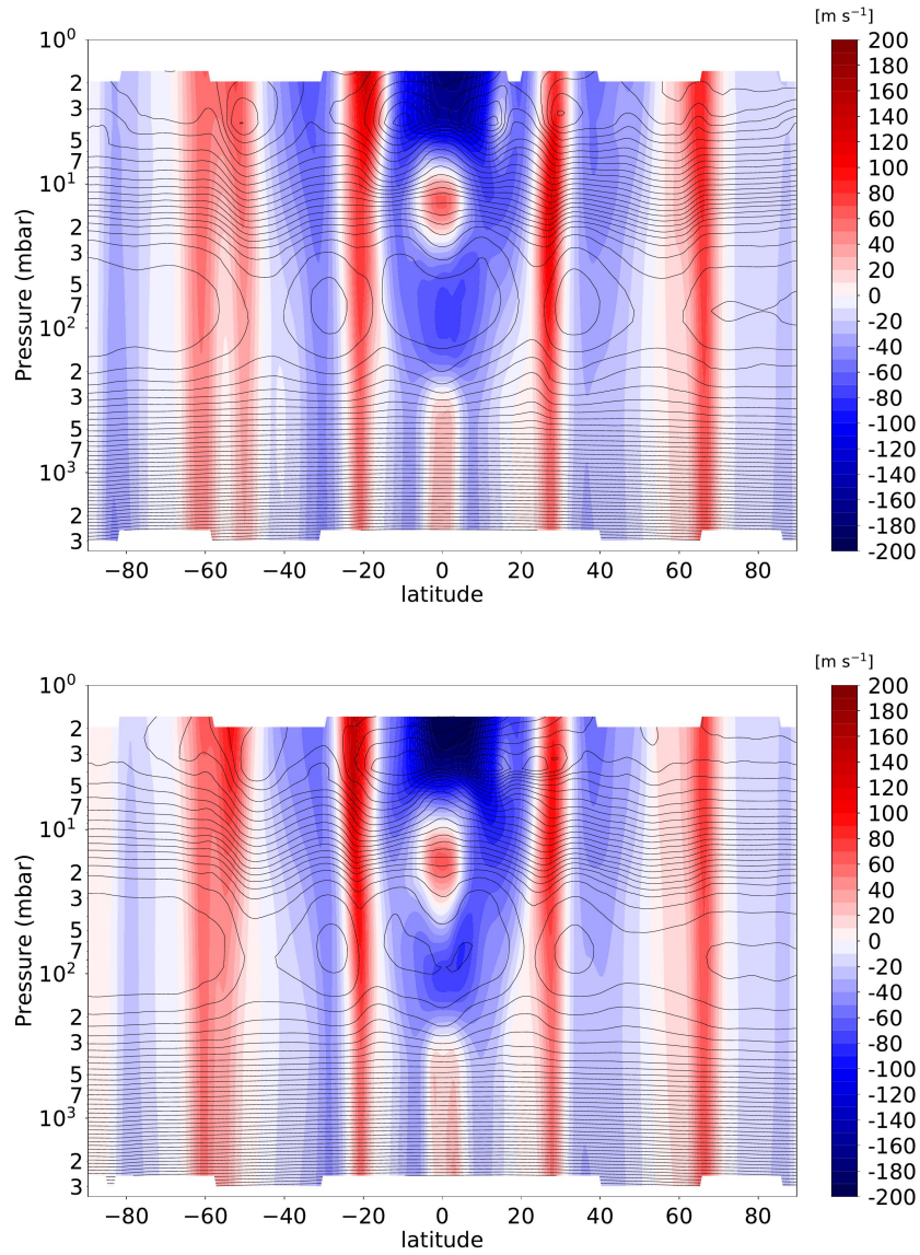
Figure 9: Same as Figure 7 for northern summer solstice ( L_s \sim 90^\circ , top panel) and fall equinox ( L_s \sim 180^\circ , bottom panel).
