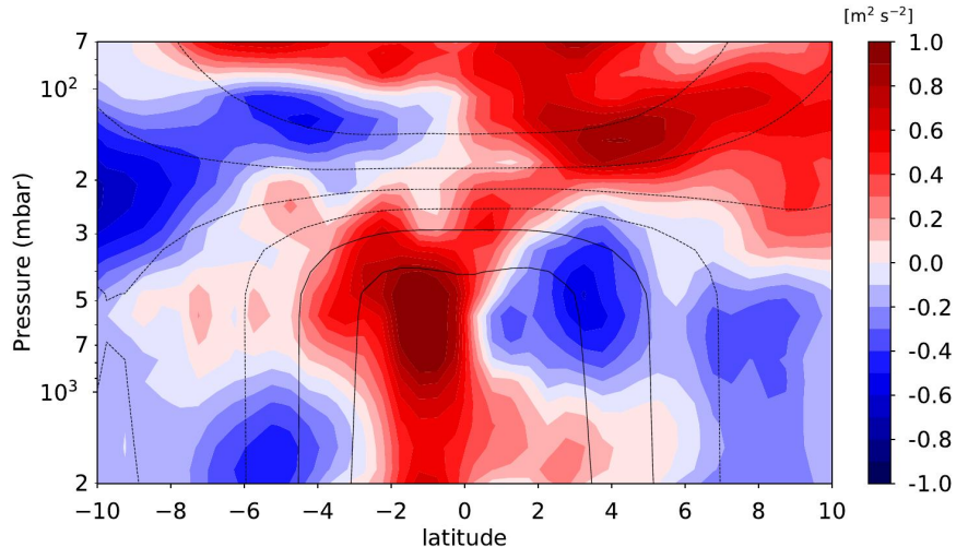
Figure 8: Latitude-pressure cross-section of zonal-mean eddy momentum transport \overline{u'v'} (colors) and zonal wind \bar{u} (contours) averaged over the whole 15-year duration of the reference simulation. This temporal averaging is carried out because, contrary to other jets, the equatorial jet does not migrate with time and the equatorial eddies develop continuously rather than through “bursts” (see Figure 13 in section 4).
