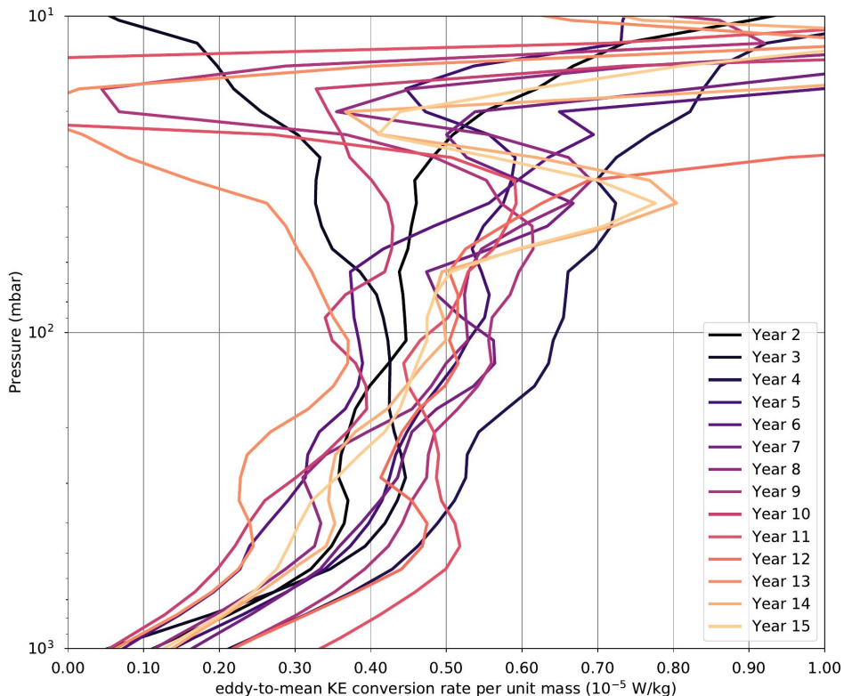
Figure 16: Rate per unit mass \mathcal{C} in \text{m}^2 \text{s}^{-3} (or \text{W kg}^{-1} ) estimating the conversion of eddy kinetic energy to zonal-mean kinetic energy. Vertical profiles of \mathcal{C} are shown, annually-averaged (one line per simulated year, from year 2 to 15) and globally-averaged ( 60^\circ\text{S} to 60^\circ\text{N} latitudes) This spatial and seasonal averaging is chosen to allow a direct comparison with Cassini estimates of \mathcal{C} in Del Genio and Barbara (2012).
