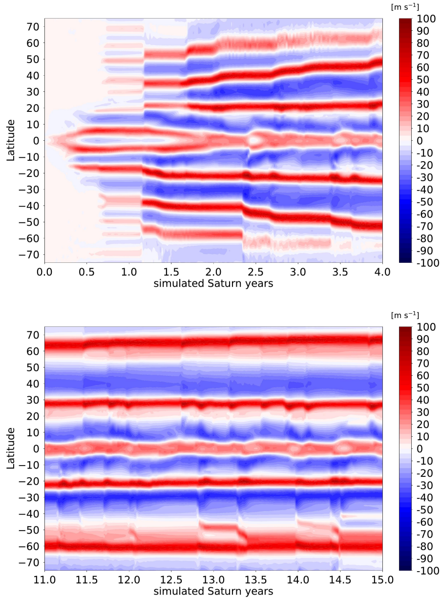
Figure 14: Same as Figure 13 with an emphasis on (top) the first four and (bottom) the last four simulated Saturn years of the full 15-year duration of our Saturn DYNAMICO GCM simulation.
