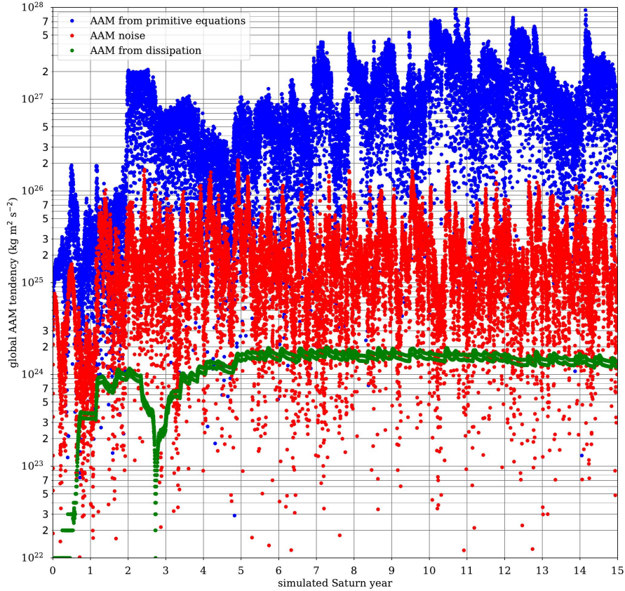
Figure 23: Temporal evolution of the tendency dM/dt of global AAM for the complete duration of our reference Saturn GCM simulation. Blue points depict the term [dM^w/dt]_{PE} associated with wind tendencies computed in the primitive equations resolved in the dynamical core of the Saturn GCM. Red points depict the term \varepsilon associated with AAM noise, i.e. residual numerical rate of AAM variation due to conservation errors. Green points depict the term D associated with AAM tendencies resulting in the dissipation and Rayleigh drag scheme. The log-scale figure is produced with the absolute values of the various tendencies dM/dt .
