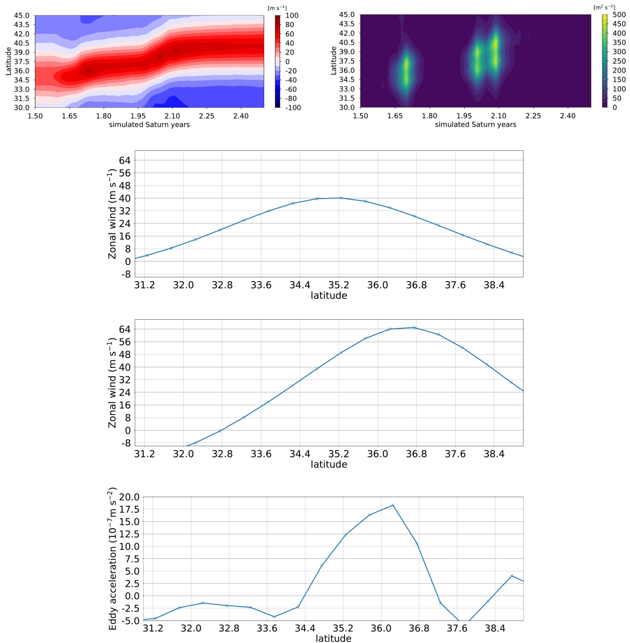
Figure 18: An episode of the poleward migration of a mid-latitude jet is shown on the top two figures offering a magnified view of a relevant portion of Figure 13 showing an episode of jet migration. The latitudinal profiles of the zonal-mean zonal jet at the beginning and in the end of the temporal interval spanned by the top plots are shown as middle plots (pressure level is 200 mbar). The bottom plot features the acceleration term obtained by equation 13 (computation of the divergence of the Eliassen-Palm flux).
