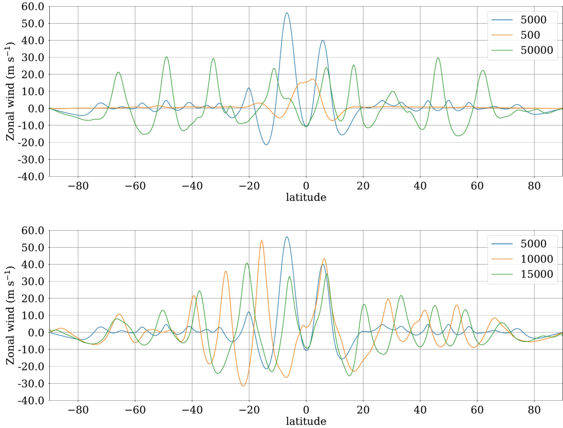
Figure 21: Zonal-mean jets obtained at cloud level after 20000 integrated Saturn days (about one simulated Saturn year) with our Saturn DYNAMICO GCM run at a horizontal resolution of 1/2^\circ . Those tests were carried out with a preceding, slightly different, version of the DYNAMICO model compared to the one used for the reference simulations of section 3. In the top plot, results are shown for three values of horizontal dissipation timescales varying by one order of magnitude (orange: strong \tau_D = 500 s, blue: moderate \tau_D = 5000 s, green: weak \tau_D = 50000 s). In the bottom plot, results are shown for three values of horizontal dissipation timescales, two of them (blue: \tau_D = 5000 s, green: \tau_D = 15000 s) enclosing the value chosen for the reference simulation discussed in sections 3 and 4 (orange: \tau_D = 10000 s).
