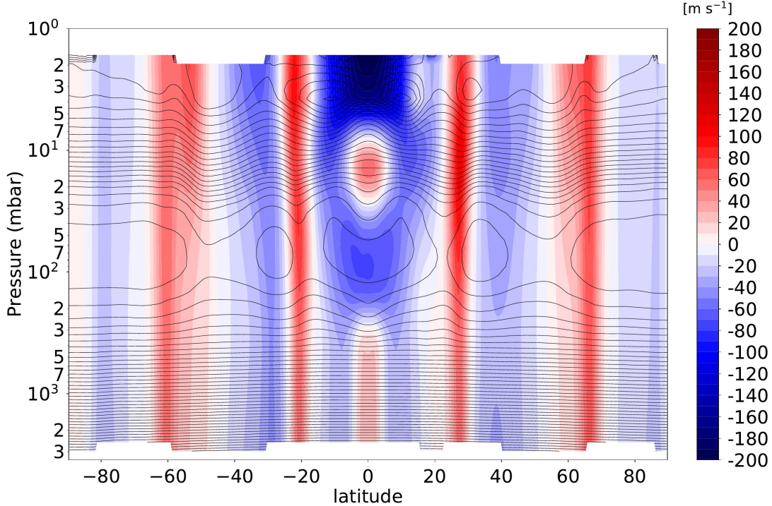
Figure 7: Instantaneous latitude-pressure cross-section of zonal-mean zonal wind \bar{u} (colors) and zonal-mean temperature \bar{T} (contours) in the beginning ( L_s \sim 0^\circ ) of the fifteenth simulated year (after about 342 thousands simulated Saturn days). Model results are similar should any of the simulated Saturn year starting from year eight be considered.
