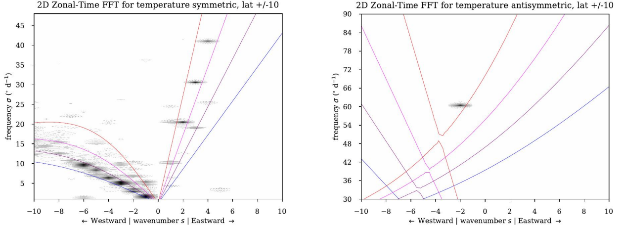
Figure 11: Spectral analysis of the equatorial waves produced in our Saturn DYNAMICO GCM (in dynamical steady-state) at the same vertical level as Figure fig:eqwave. This spectral power mapping is obtained by a two-dimensional Fourier transform from the longitude \lambda / time t space to the zonal wavenumber s / frequency \sigma space (Wheeler and Kiladis, 1999) of the symmetric component of temperature T_S about the equator (left, see equation 3) and antisymmetric component of temperature T_A about the equator (right). We follow the common assumption of a positive sign convention for frequency \sigma , meaning that s > 0 modes are eastward-propagating and s < 0 modes are westward-propagating. The dispersion relation for equatorial waves (equation 4) is superimposed for meridional mode number \nu = -1, +1 (left panel, Rossby waves on the s < 0 side and Kelvin waves on the s > 0 side) and meridional mode number \nu = 0 (right panel, Yanai waves on the part of the curves increasing with s ). Four values of equivalent depths (equation 5) are included: h = 5 km (blue), h = 10 km (purple), h = 20 km (magenta), h = 50 km (red).
