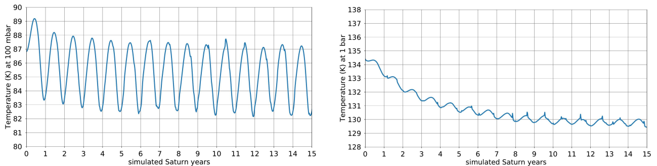
Figure 1: Evolution over the whole 15-year duration of the reference Saturn GCM simulation of zonal-mean temperature \bar{T} , averaged over latitudes \varphi = 20 - 60^\circ N , in the tropopause region ( p = 100 mbar, left) and in the troposphere ( p = 1 bar, right).
