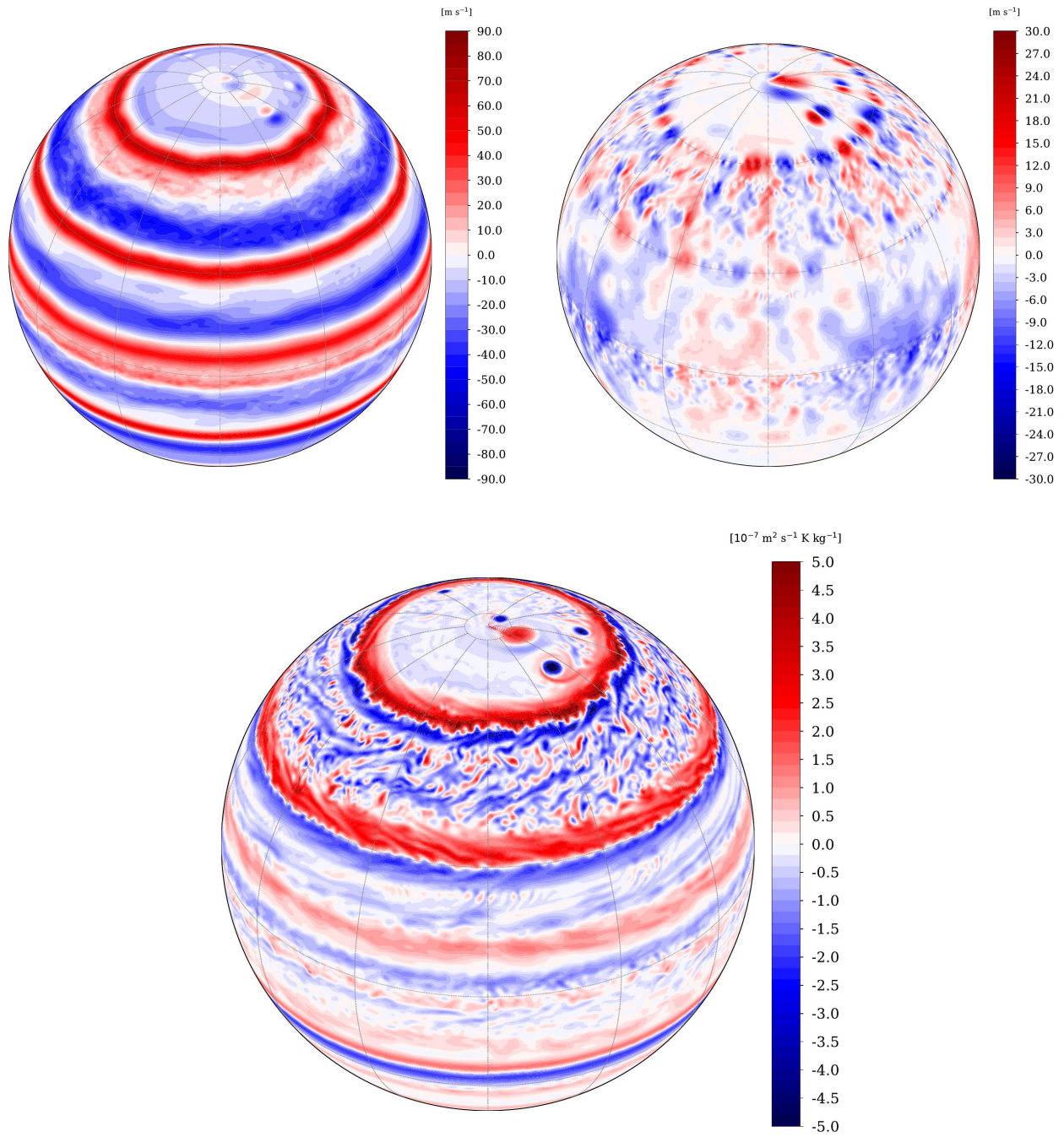
Figure 12: Instantaneous view on (top left panel) the zonal wind u and (top right panel) the meridional wind v on the fifth sigma level of the model (pressure level \sim 1.5 bar), as in Figure 5 and (bottom panel) relative Ertel potential vorticity (PV) on tropospheric isentrope \theta = 205 K after 171 thousands simulated Saturn days (beginning of the seventh simulated year). Ertel PV computations are described in equation 1 and section 3.2.1.
