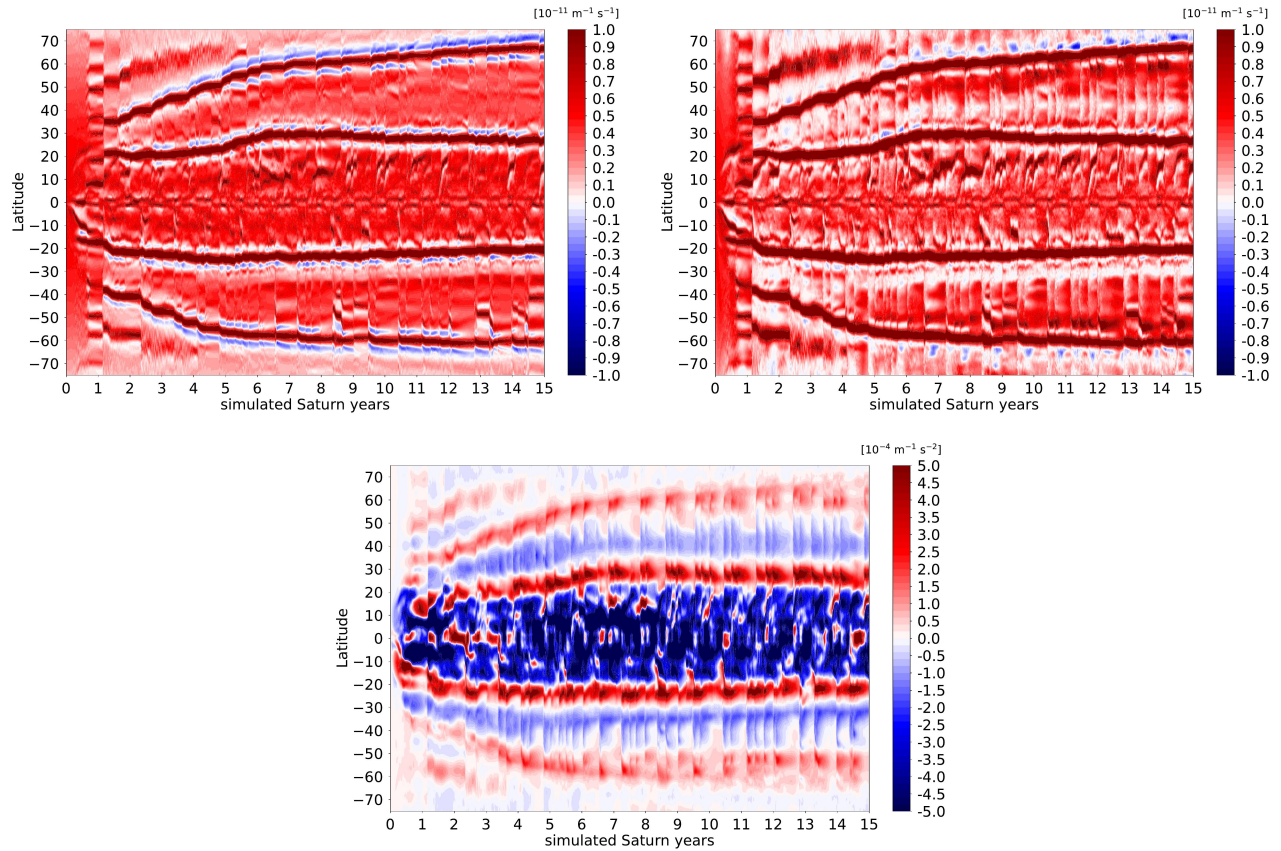
Figure 19: Evolution of the meridional gradients of zonal-mean potential vorticity (top left: barotropic, equation 14 for necessary condition RK, top right: baroclinic, equation 15 for necessary condition CSP1) and vertical shear of zonal-mean zonal wind (bottom) at Saturn’s tropopause (100 mbar) within the whole 15-year duration of our Saturn DYNAMICO GCM simulation. The diagnostic in equation 14 cannot be computed in the troposphere where the atmosphere is neutral ( N^2 \sim 0 ) and barotropic; the two other diagnostics are shown at the tropopause for consistency but are similar at deeper levels.
