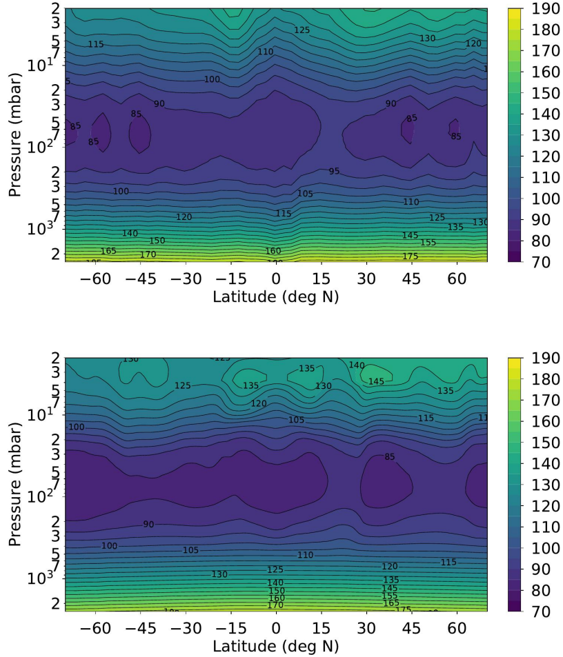
Figure 2: Latitude-pressure section of zonal-mean temperature \bar{T} (top) observed by Cassini/CIRS in 2015 (Guerlet et al., 2015a) vs. (bottom) produced by our Saturn DYNAMICO GCM in the fourteenth simulated Saturn year at L_s \sim 70^\circ (see Table 1 for a definition of L_s ). The Cassini/CIRS observations shown here are nadir retrievals, with optimal sensitivity in the 500 – 70 mbar and 5 – 0.5 mbar ranges. Model results are similar should any of the simulated Saturn year starting from year eight be considered.
