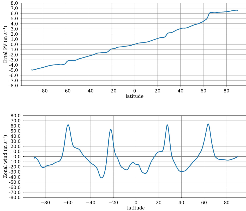
Figure 6: Instantaneous zonal-mean Ertel potential vorticity (top) and zonal wind (bottom) projected on a surface of equal potential temperature 205 K, corresponding to tropospheric conditions. The time adopted for this plot is similar to Figure 5. The 205 K value of potential temperature corresponds to upper tropospheric conditions, higher in altitude than Figure 5; lower tropospheric conditions are not accessible through this diagnostic due to the difficulty of defining the Ertel potential vorticity on isentropes in neutral conditions ( N^2 \sim 0 ). Our Python code used to calculate potential vorticity contains excerpts from the code by Barlow (2017).
