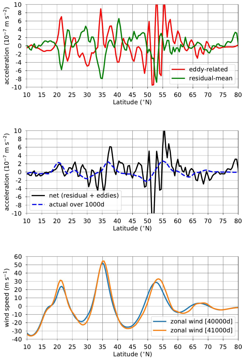
Figure 17: Meridional profiles of the zonal-mean acceleration terms in the Eulerian-mean formalism described by equation 9. The analysis is carried out after 41 thousands simulated Saturn days (around 1.6 simulated year), corresponding to a typical burst of eddies in the northern hemisphere evidenced in Figure 13. The plots are obtained after averaging over 1000 Saturn days. The residual-mean term (equation 10) is shown in the red line and the eddy-related term (equation 11) is shown in the green line. The net resulting acceleration is shown in the black full line and the actual acceleration obtained within the considered 1000 days is shown in the dashed blue line. The comparison of the latitudinal profiles of zonal-mean zonal winds at the beginning and in the end of the 1000-day sequence are shown respectively in light blue and orange in the bottom plot.
