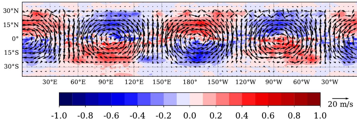
Figure 10: Instantaneous view on the zonal perturbations of temperature T' (shaded contours) and horizontal winds [u', v'] (wind vectors) in the beginning ( L_s \sim 0^\circ ) of the twelfth simulated year (after 270 thousands simulated Saturn days), on the fifteenth sigma level of the model (pressure level \sim 130 mbar, corresponding to Saturn's tropopause, transition between troposphere and stratosphere). Only latitudes below 40^\circ N/S are shown (tropical channel). A similar figure is obtained at Saturn's cloud level ( \sim 1.5 bar, as in Figure 5), with an even stronger prominence of the wavenumber-2 signal.
