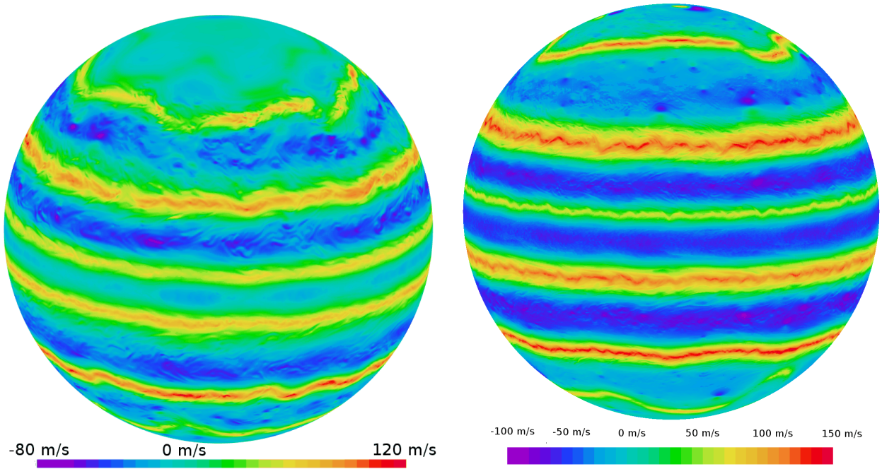
Figure 20: Instantaneous zonal winds predicted at 0.5 bar (yellow/red: prograde jets, blue/violet: retrograde jets) after 500 simulated Saturn days by our Saturn DYNAMICO GCM. Our simulations used a horizontal resolution of 1/4^\circ (left) and 1/8^\circ (right) longitude, and extent from troposphere to the stratosphere. In the left plot, jets’ instabilities and filamentation can be noticed; in the right plot, the even finer horizontal resolution allows the model to reproduce the propagation of gravity waves on the flanks of the jets, as well as the possible emergence of traveling vortices (cf. blue/green spots in the northern hemisphere). The objectives behind those simulations were more technical (testing a massively-parallel computing cluster) than scientific: the strong hyperdiffusion made the structures seen in the figure to disappear after about a thousand simulated Saturn days.
