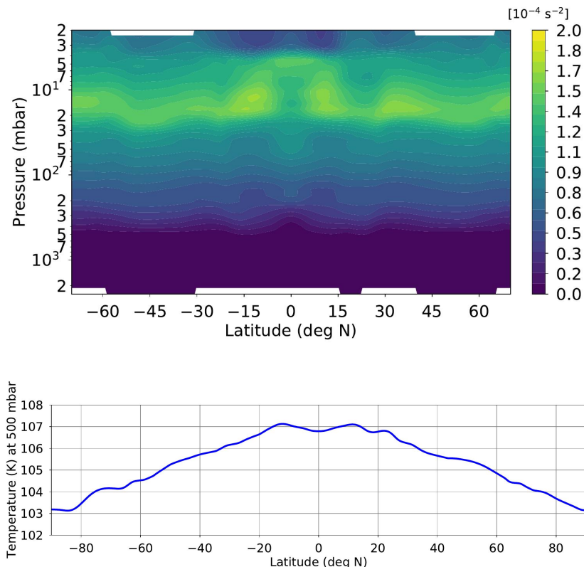
Figure 3: (Top) Latitude-pressure section of zonal-mean Brunt-Väisälä frequency \overline{N^2} and (bottom) meridional profile of zonal-mean temperature \overline{T} at 500 mbar, averaged over the fourteenth simulated Saturn year with our Saturn DYNAMICO GCM.
