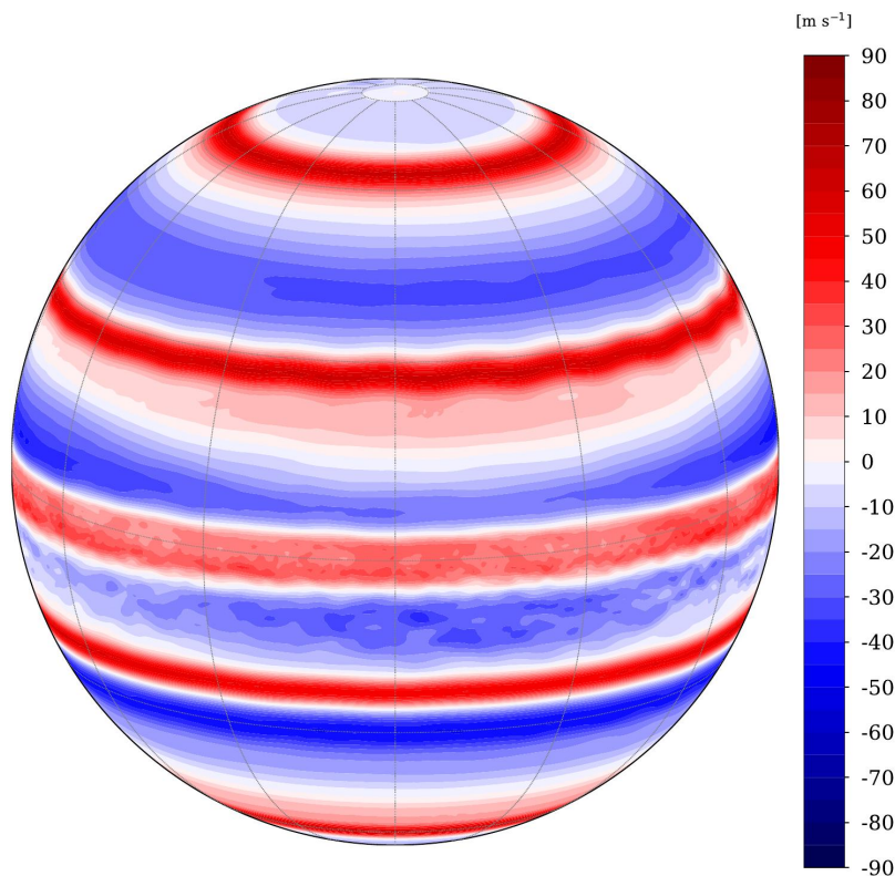
Figure 5: Instantaneous zonal wind u in the beginning ( L_s \sim 0^\circ ) of the twelfth simulated year (after 270 thousands simulated Saturn days), on the fifth sigma level of the model (pressure level \sim 1.5 bar, corresponding to Saturn’s visible cloud deck and tropospheric conditions).
