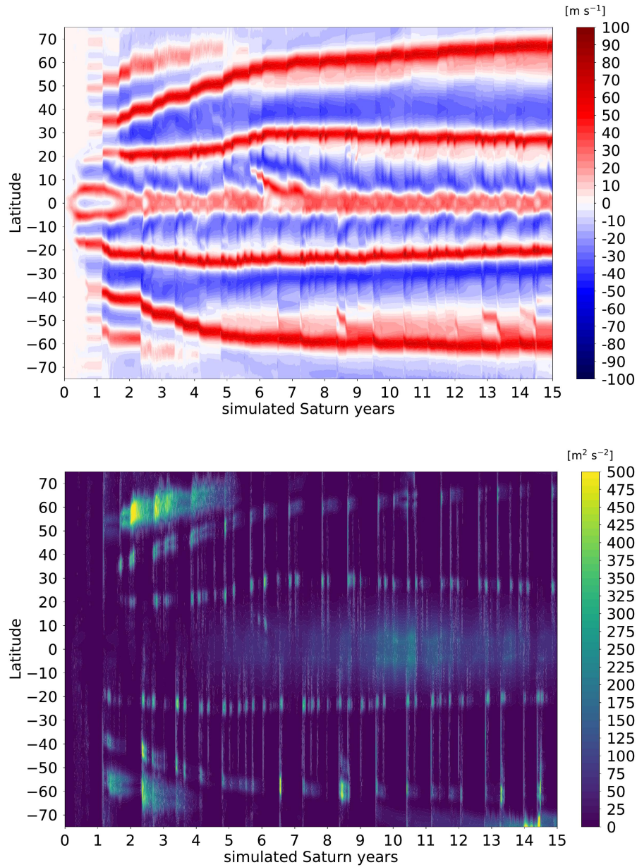
Figure 13: Evolution of the zonal-mean zonal wind \bar{u} (top plot) and the zonal mean of the Eddy Kinetic Energy (EKE) 1/2(u'^2 + v'^2) (bottom plot) in Saturn troposphere (800 mbar) within the whole 15-year duration of our Saturn DYNAMICO GCM simulation.
