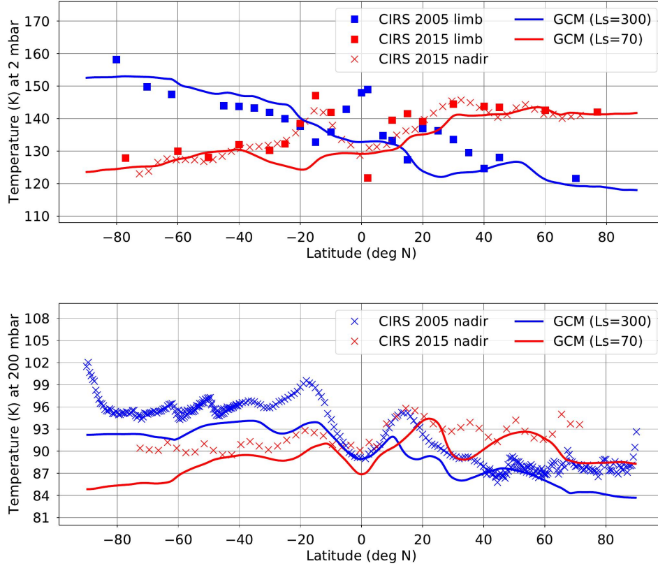
Figure 4: Meridional profiles of zonal-mean temperature \bar{T} at the two opposite solstices explored by the Cassini spacecraft (blue: year 2005, L_s = 300^\circ ; red: year 2015, L_s = 70^\circ ). Squares correspond to Cassini / CIRS limb retrievals (Guerlet et al., 2009, 2015a), crosses correspond to Cassini / CIRS nadir retrievals (Fletcher et al., 2007; Guerlet et al., 2015a), lines correspond to Saturn DYNAMICO GCM simulations (fourteenth simulated year). Middle stratospheric conditions (2 mbar) are shown in the top plot, where both CIRS limb and nadir retrievals are valid; upper tropospheric conditions (200 mbar) are shown in the bottom plot, where CIRS nadir retrievals are valid. Model results are similar should any of the simulated Saturn year starting from year eight be considered.
