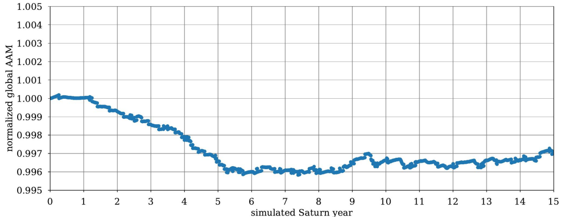
Figure 22: Temporal evolution of the global AAM \mathcal{M} (normalized to the initial value \mathcal{M}_0 = 5.244 \times 10^{32} \text{ kg m}^2 \text{ s}^{-1} ) for the complete duration of our reference Saturn GCM simulation.
