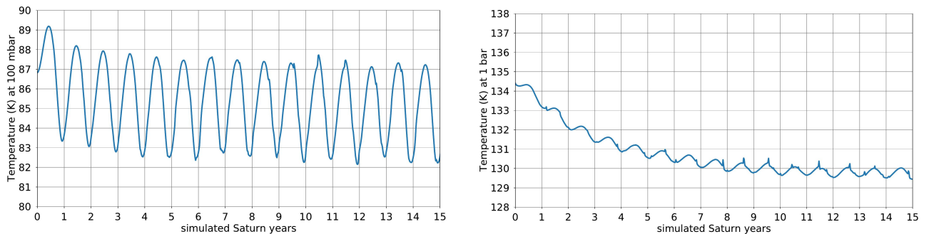
Figure 1: Evolution over the whole 15-year duration of the reference Saturn GCM simulation of zonal-mean temperature \bar{T} , averaged over latitudes \varphi = 20 - 60^\circ N , in the tropopause region ( p = 100 mbar, left) and in the troposphere ( p = 1 bar, right).
