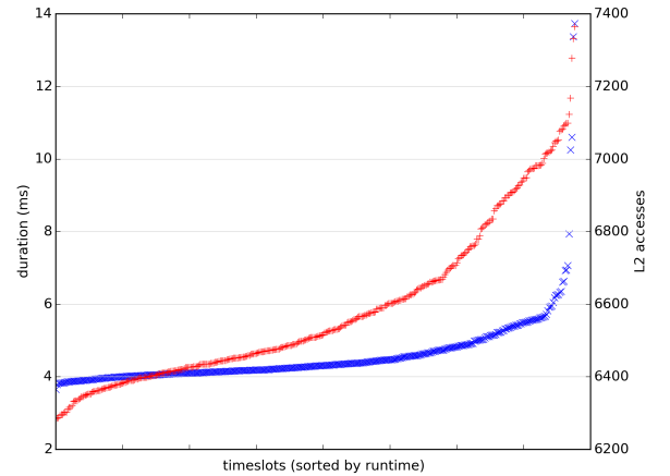
Fig. 9. Variation of the runtime (in blue x) and L2 accesses (in red +) while running the FMS application standalone
