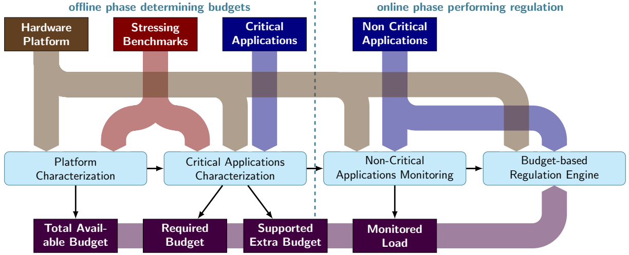
Fig. 3. Timing integrity process for mixed time-critical systems
