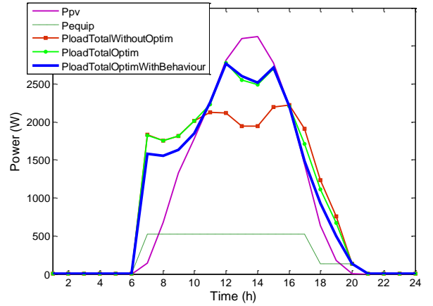
Figure 10. Controlled load power with and without management.
