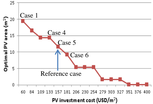
Figure 7. Optimal size of PV as a function of the unit investment cost of solar panels.
