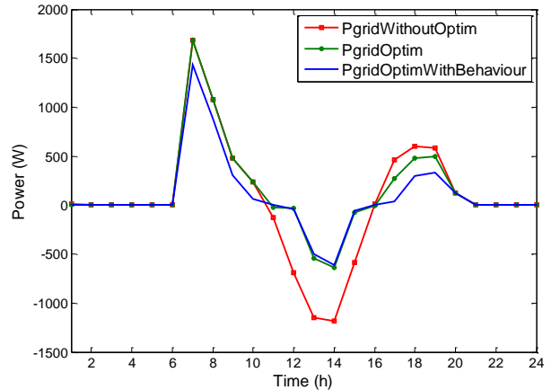
Figure 11. Grid power with and without management.
