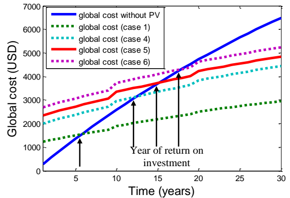
Figure 8. Time duration for return on PV investment.
