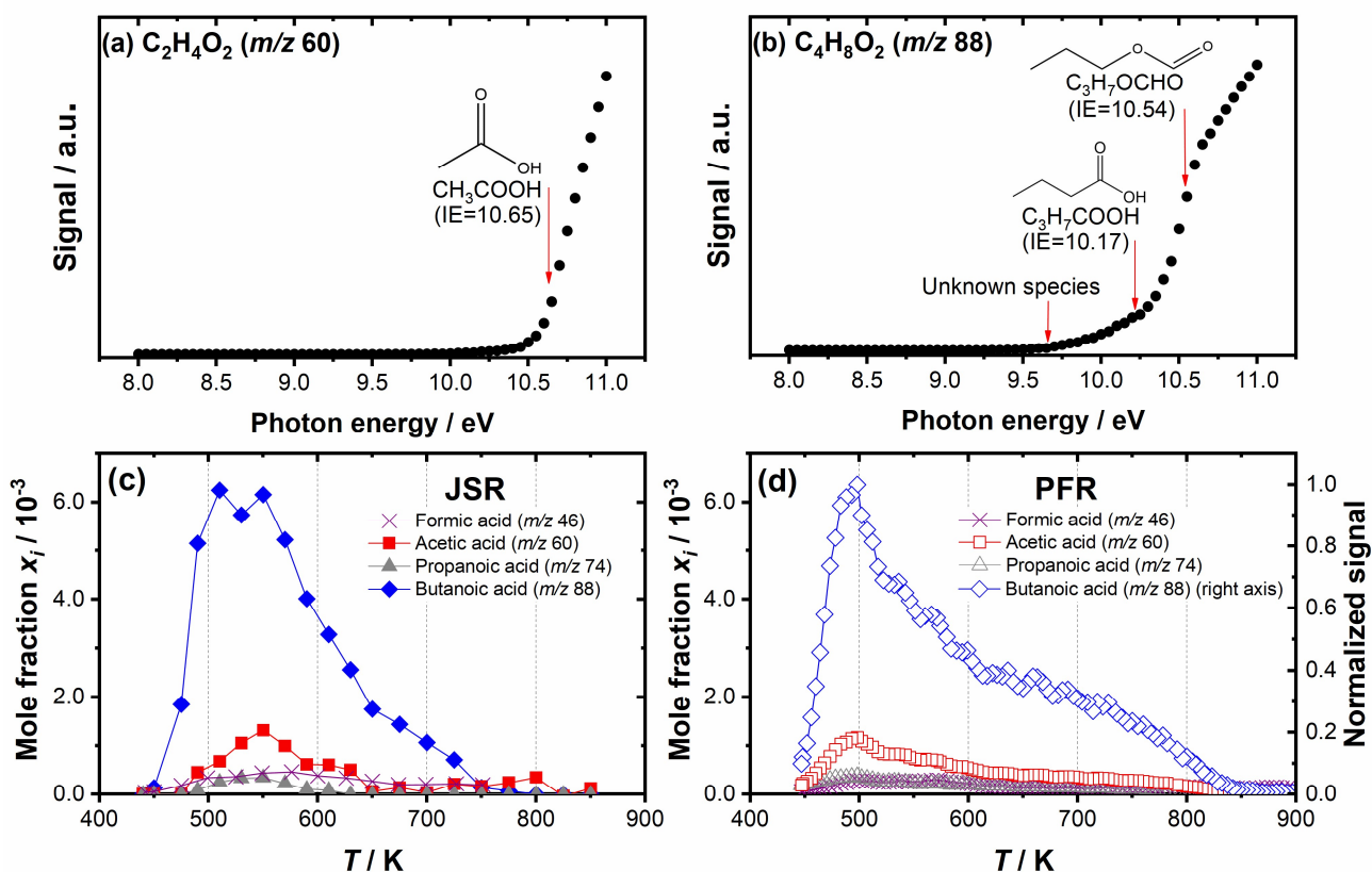
Figure 6. PIE curves at 500 K from the JSR-PI-MBMS experiment for m/z 60 (a) and 88 (b), corresponding to acetic acid (CH 3 COOH) and butanoic acid (C 3 H 7 COOH), respectively. Profiles of the detected acids; (c) JSR, (d) PFR.
