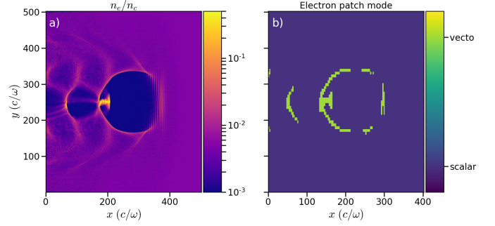
Figure 14: Laser wakefield acceleration with 4 PPC. Same as Fig. 13 but taking a 2D slice at z = 0.5 L_z ( L_z being the domain length in the z direction) a) Electron charge -n_e/n_c at time t = 2770 \omega^{-1} . b) Patches using a vectorized operator for the electron species at the same time.
