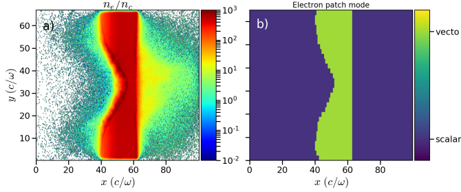
Figure 17: Laser over-dense foil interaction. a) Slice at z = 0.5L_z of the electron density n_e/n_c at time t = 475\omega^{-1} corresponding to the end of the laser interaction. b) Patches using a vectorized operator (adaptive mode) for the electron species at the same time..
