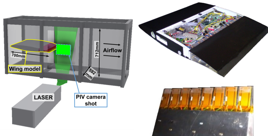
Figure 1: Schematic representation of the experimental test section of the S4 wind tunnel of IMFT (left) with the Airbus-A320 wing (right-top) mounted on [5]; the prototype bears the HFVTE actuators (right-bottom) on the trailing edge along the span.
