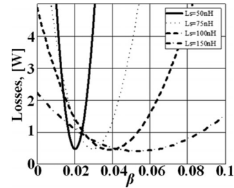
Fig. 4. Total losses ( V_{IN} = 5 \text{ V} , f_{sw} = 1 \text{ MHz} , and R = 2.5 \text{ } \Omega ).
