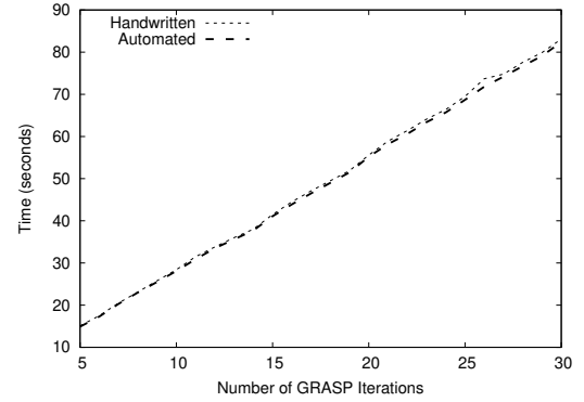
Figure 6: Skeleton overhead for sequential execution
