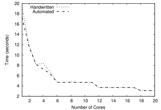
Figure 7: Skeleton overhead for parallel execution
