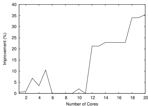
Figure 9: One-level vs two-level orchestrations
