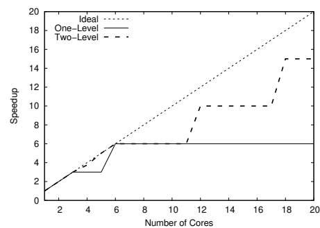
Figure 5: Theoretical speedup of two-level orchestration
