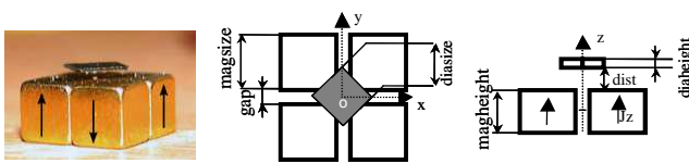
Fig. 10: Geometrical parameters of magnets and diamagnetic ball.
