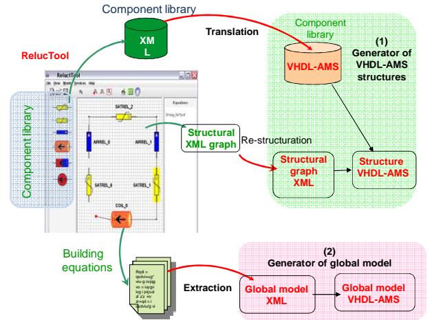
Fig. 5: VHDL-AMS translation methodology from Reluctool
