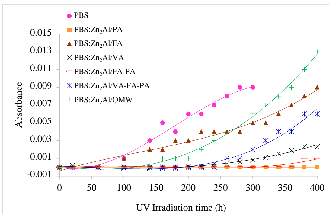
Figure 9: Kinetic curves of hydroxylated photo-products from oxidation of PBS (the film was destroyed after 300 h) and its composites: evolution of hydroxyl absorbance at 3260\text{ cm}^{-1} as a function of photoageing time at \lambda > 300\text{ nm} at 60\text{ }^\circ\text{C} .
