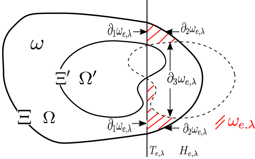
Figure 4: The three parts \partial_1\omega_{e,\lambda} , \partial_2\omega_{e,\lambda} and \partial_3\omega_{e,\lambda} of the boundary of the set \omega_{e,\lambda} (dashed red)
