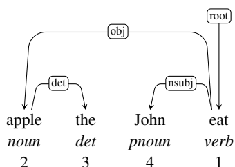
(a) Unordered Source Tree
