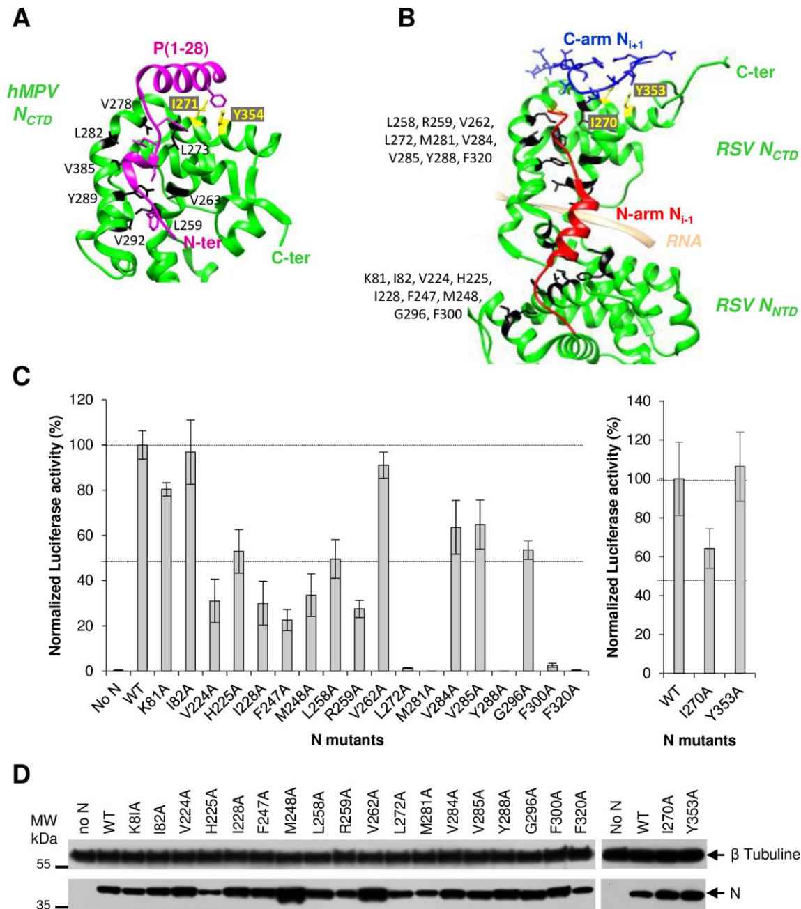
Figure 2: Search for the P40 binding site at the surface of N. (A) Ribbon representation of the hMPV N_{CTD} (green) in interaction with the peptide of P (residues 1-28, purple). The residues of N involved in the interaction with P are colored in black and yellow and the side chains are shown (PBD code 5FVD) (B) Ribbon representation of a part of RSV N protomer (green) from N-RNA 3D crystal structure (PBD code 2WJ8) showing binding of the N_{i-1} N-arm (in red) and of the N_{i+1} C-arm (in blue). Residues involved in N_{i-1} N-arm or in N_{i+1} C-arm binding, and that could also interact with P40, are colored in black and yellow, respectively, and their side chains are shown, (C) Effect of N mutations on RSV polymerase activity. BSRT7/5 cells were transfected with plasmids encoding the WT P, M2-1 and L proteins, the pMT/Luc minigenome, and WT or mutant N proteins, together with pCMV- \beta Gal for transfection standardization. Viral RNA synthesis was quantified by measuring the luciferase activity after cell lysis 24 h after transfection. Each luciferase minigenome activity value was normalized based on \beta -galactosidase expression and is the average of three independent experiments performed in triplicate. Error bars represent standard deviations calculated based on three independent experiments made in triplicate. (D) Western blot showing the expression of N protein variants in BSRT7/5 cells.
