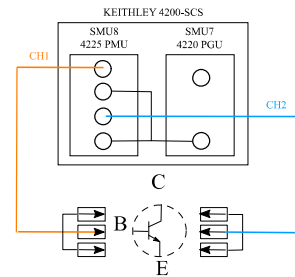
Fig.8 : Measurement test bench for pulse measurements
