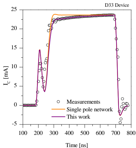
Fig. 10 : D33 device comparison between measurements (symbols) and HiCuM compact model simulation results using single pole network (orange lines) and physics based multi-pole network (purple lines) at T_W=500ns , V_{BE}=0.95V and V_{CE}=1.5V
