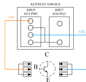
Fig.8 : Measurement test bench for pulse measurements
