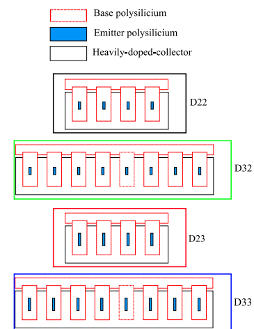
Fig.2 : Layout view for BEC configuration of DUTs
