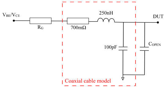
Fig.9: Passive network including coaxial cables, generator resistance R_G and device open capacitance C_{OPEN}
