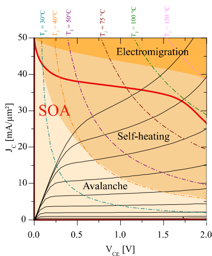
Fig.1 : Safe-Operating-Area definition for HBT
