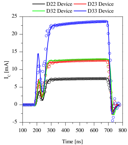
Fig.11 : Comparison between HiCuM compact model transient simulation and waveform captures for at T_W=500ns , V_{BE}=950mV and V_{CE}=1.5V the collector current I_C for all device geometries
