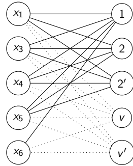
(a) Lower Bound Graph after adding fake vertices, G_I^{bal} .
