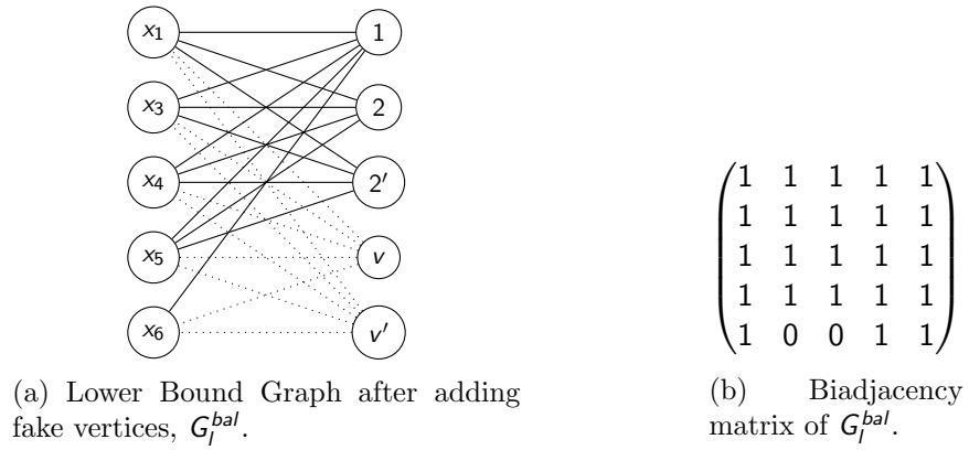
Figure 4: Lower Bound Graph after adding fake vertices and its biduality matrix.
