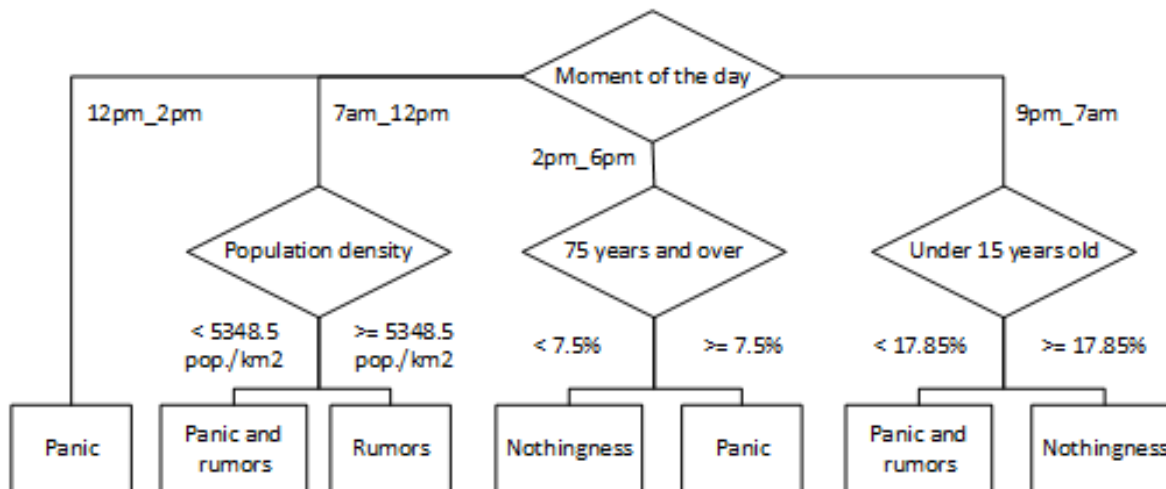
Figure 3: Decision tree obtained with the algorithm Random Tree
