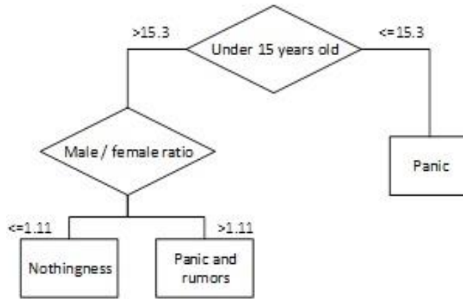
Figure 2: Decision tree obtained with the algorithm J48-C4.5
