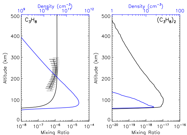
Figure 10. Simulated propane C_3H_8 and propane dimer (C_3H_8)_2 abundances in Titan's lower atmosphere. Black lines represent the mixing ratios and blue lines the corresponding number densities of each component. The gray and black curves with error bars correspond to the retrieved C_3H_8 stratospheric abundance from Cassini observations at mid latitudes (30N and 39N, respectively, from Vinatier et al. 2010 ), which are more representative of our disk-averaged simulations.
