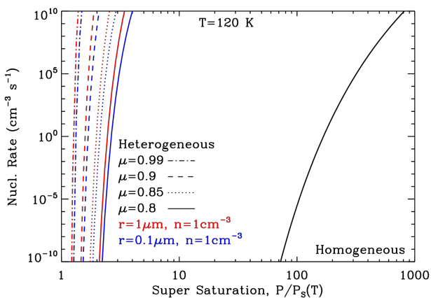
Figure 11. Predictions of classical nucleation theory for the homogeneous (black line) and heterogeneous (red and blue lines) nucleation rates of C_3H_8 . Different colours present evaluations of heterogeneous nucleation rates at different radius spherical particles, while different broken lines reveal the dependence of the heterogeneous rate on the contact angle between the condensate and the substrate.
