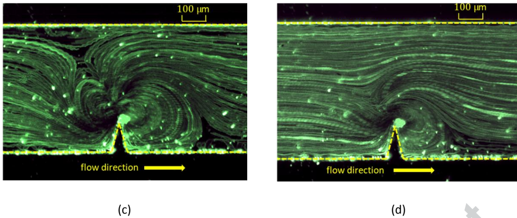
(c) (d) Figure 9: Flow visualization near the sharp tip, using particle trajectories at different channel throughputs, experimental conditions: \alpha = 30^\circ , V_a = 101.7 mm/s and f = 2.5 kHz. The flow direction is from left to right.
