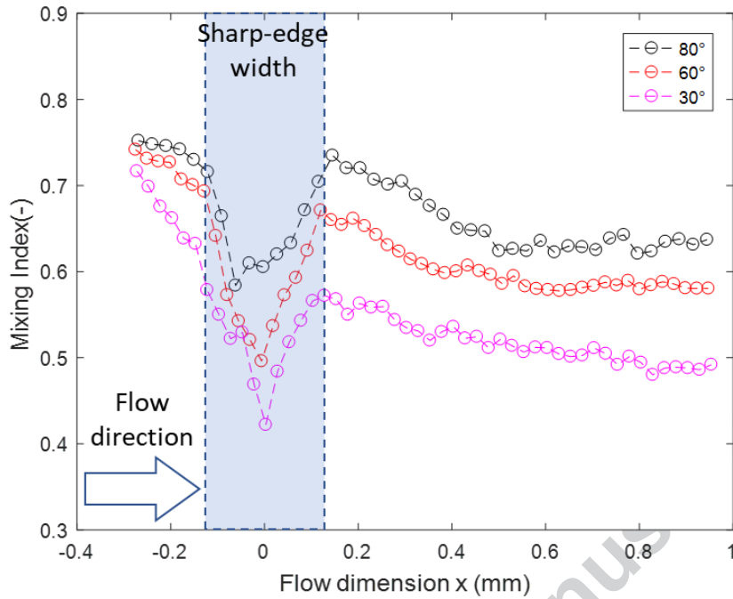
Figure 15: Mixing Index at different tip angles of the sharp edges. Conditions: V_{\omega} = 70.5 \text{ mm/s} and f = 2.5 \text{ kHz} , Q_s = 2 \mu\text{L/min}
