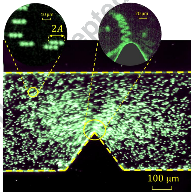
Figure 5: The mechanism of acoustic streaming explained by high-speed visualization of acoustic vibrations within the fluid, from particle trajectories over a few periods, the velocity measured is 101.7 mm/s. (see Supplementary video for dynamic visualization effect).
