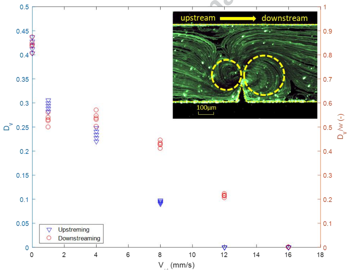
Figure 11: Upstream and downstream vortex size ( D_v and D_v/w ) at different flowrates
