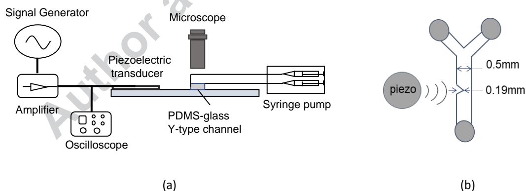
Figure 3: Sketch of the experimental setup
