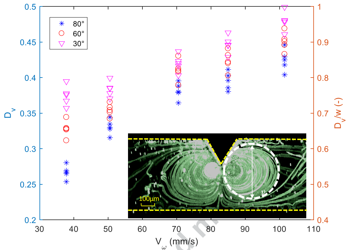
Figure 10: Vortex size D_v and its relative value to the channel width D_v/w at zero flowrate around different sharp edge angles and acoustic stimulations
