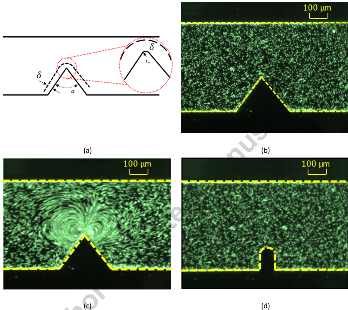
Figure 2: Mechanism of acoustic streaming under zero flowrate
