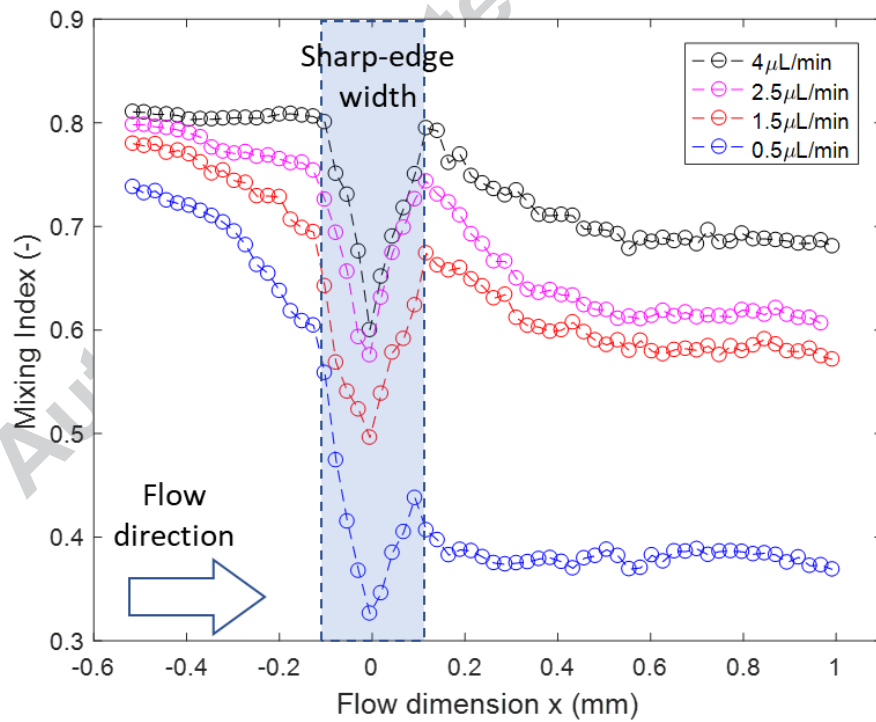
Figure 16: Mixing index at different flow rates, the values shown being those for each individual inlet.
