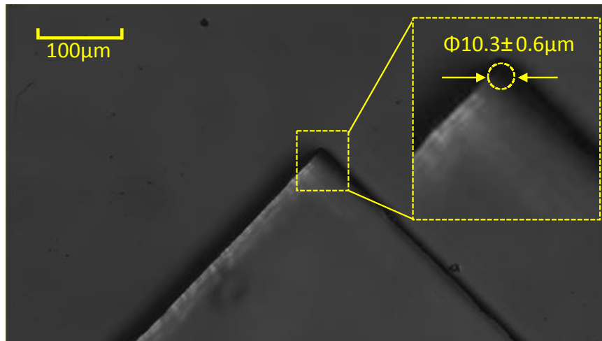
Figure 4: Measurement of the curvature diameters with 120X microscope, \alpha = 90^\circ
