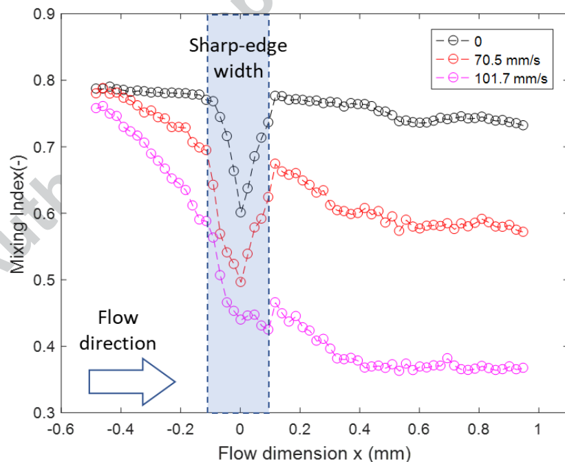
Figure 14: Mixing Index at different acoustic excitation amplitudes.
