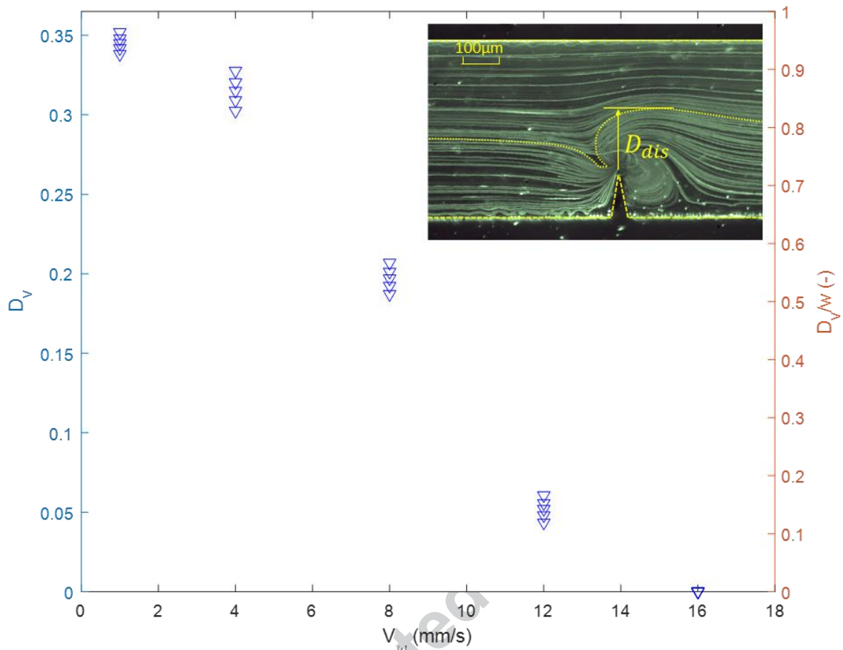
Figure 12: Disturbance extension D_{dis} as a function of channel throughput
