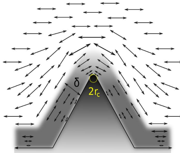
Figure 1: Sketch of acoustic oscillating flow around a tip edge
