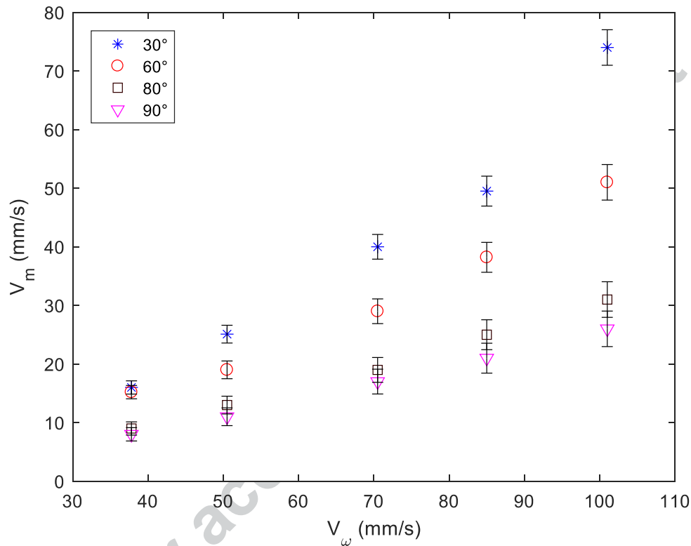
Figure 8: Maximum streaming velocity versus acoustic velocity, generated near sharp tips of different angles, under no-flow condition ( Q_c = 0 ).
