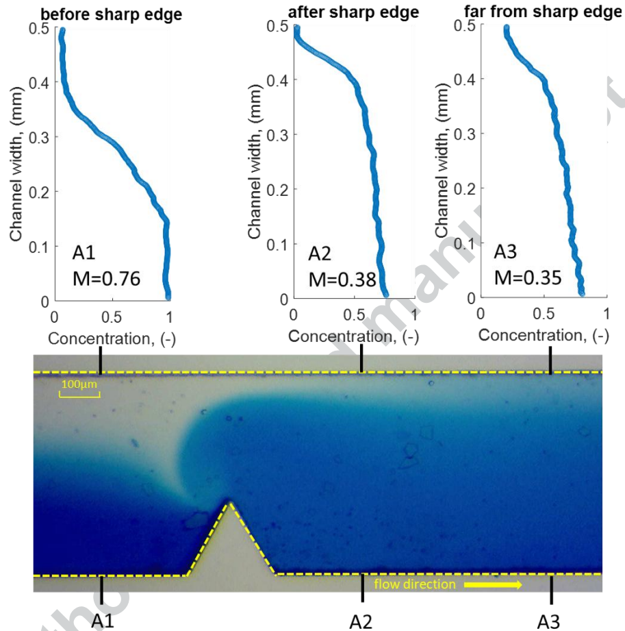
Figure 13: Concentration field across the microchannel section in the nearby area before and after the sharp edge. X axis is the normalized concentration C_n (value 0 and 1 represents two different fluids, 0.5 means complete mixing); Y axis is channel width.
