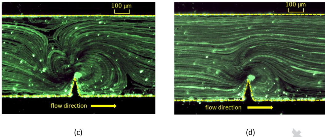
(c) (d) Figure 9: Flow visualization near the sharp tip, using particle trajectories at different channel throughputs, experimental conditions: \alpha = 30^\circ , V_a = 101.7 \text{ mm/s} and f = 2.5 \text{ kHz} . The flow direction is from left to right.
