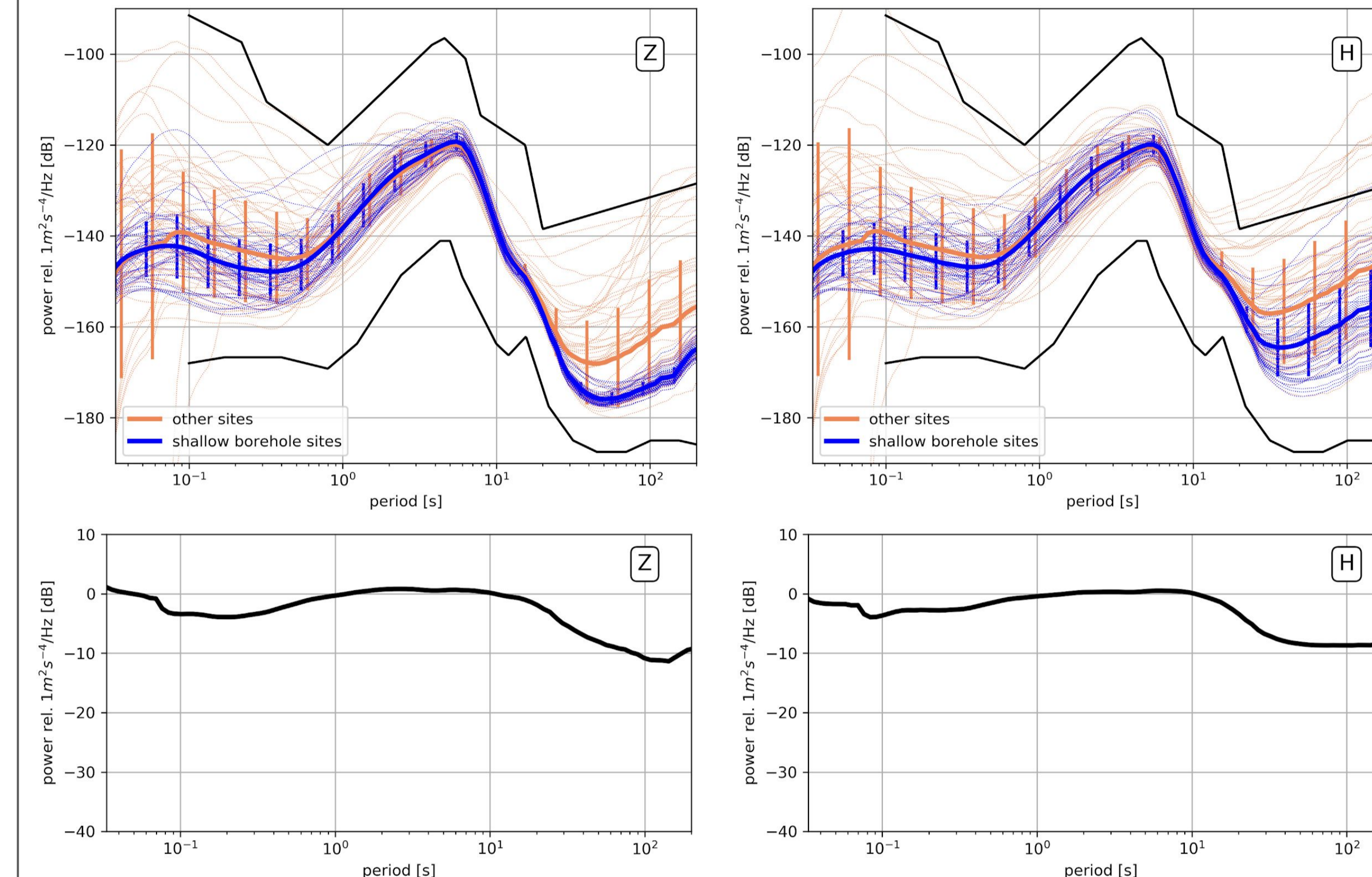
Figure 3.1 : (top) Similar to Fig 2.1 but comparing the mPDF-PSD of one month (Jan. 2019) of continuous records at RLBP operating stations installed in a shallow borehole (blue) or in other kind of "vault-like" infrastructure (orange). (bottom) Difference between the mean of the mPDF-PSD for these two kind of configuration (blue - orange curves shown on top).
