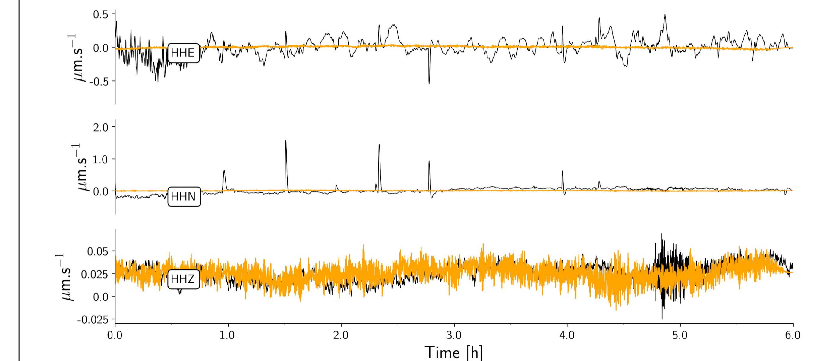
Figure 4.2 : 6 hours of filtered (lowpass at 1/20 Hz) traces at station BOUF. Solid black curves correspond to a period with no sand around the sensor and with cable issues (glitches). Solid orange curves correspond to a "well" installed sensor/cable with sand. The glitches are not detectable on the unfiltered traces but dramatically affect the noise level observed on PSD. Adding sand around the sensor has a dramatic effect of the noise level of the horizontal components at long period.
