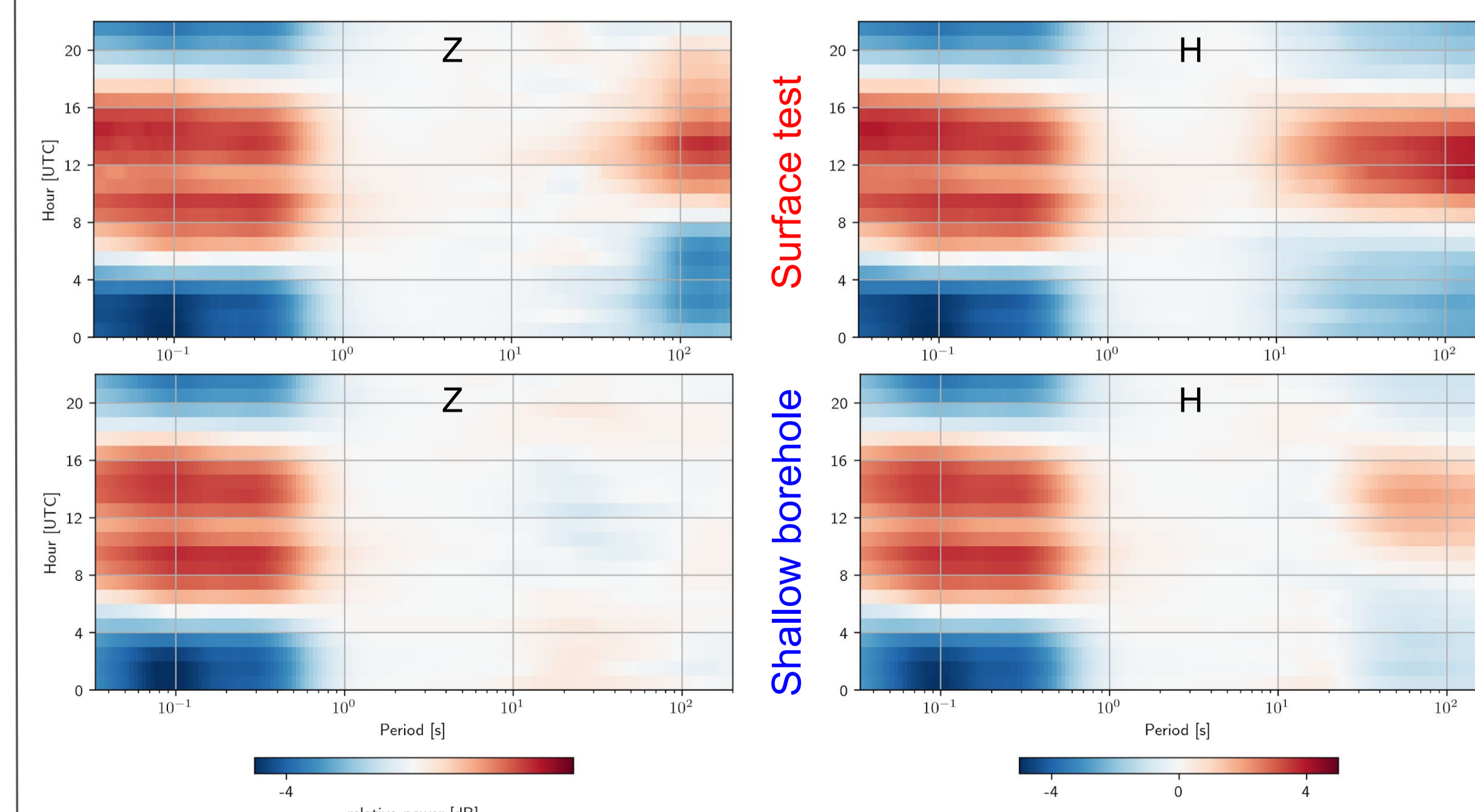
Figure 2.2 : Daily variation of ambient noise with frequency. Each of the 4 panels represents spectrograms binned by the hour of the day in UTC (local time is +1 or +2H) and after removing the mean value at each frequency. Top panels show the mean of such daily-averaged spectrograms for the 43 sites in their test configuration (left = vertical component; right = mean of the two horizontal components) and bottom panels for the shallow borehole configuration.
