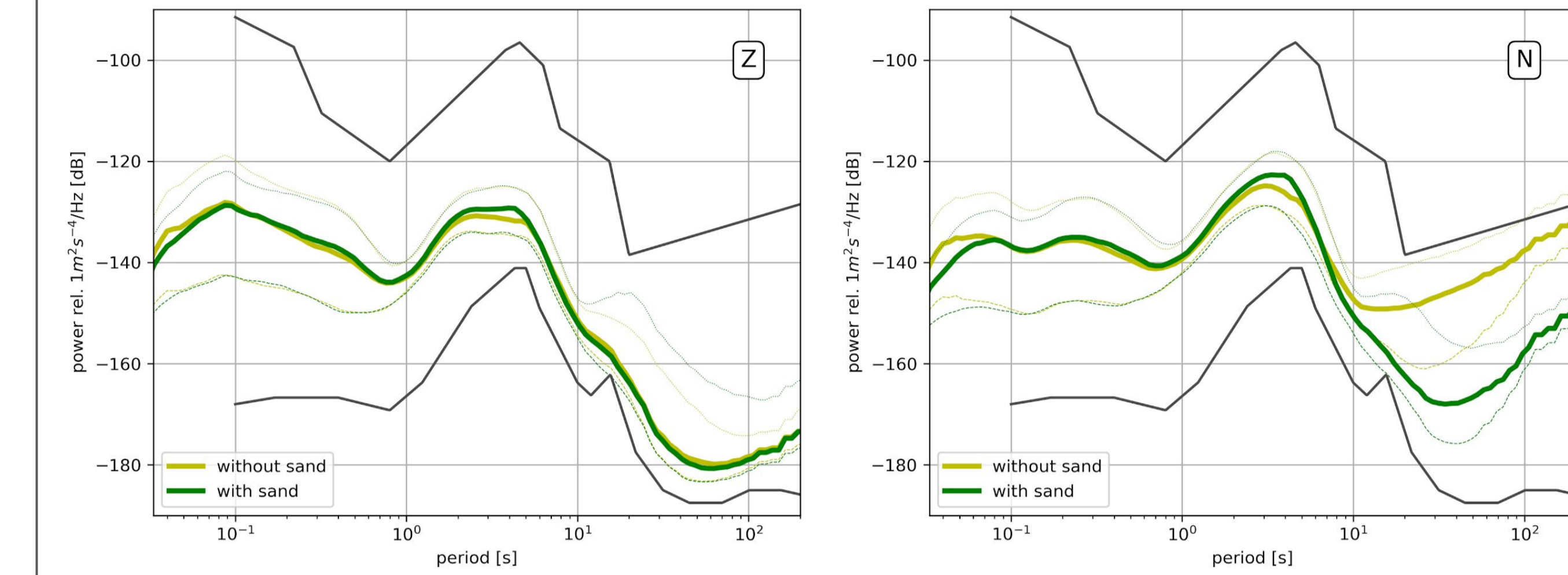
Figure 4.1 : vertical and horizontal mPDF-PSD for the station CRAS (Crastes, Gers), during two periods: - from May 30, 2018 to July 5, 2018, during which the borehole sensor was installed without sand (yellow line). - from July 21, 2018 to August 27, 2018, during which the borehole sensor was silted up (green line). Between these two periods, the sensor was not manipulated, the sand was poured into the borehole (6m) in order to cover the sensor. Heavy, dotted and dashed lines respectively indicate the mPDF-PSD, the 5th and the 95th percentiles for each period.
