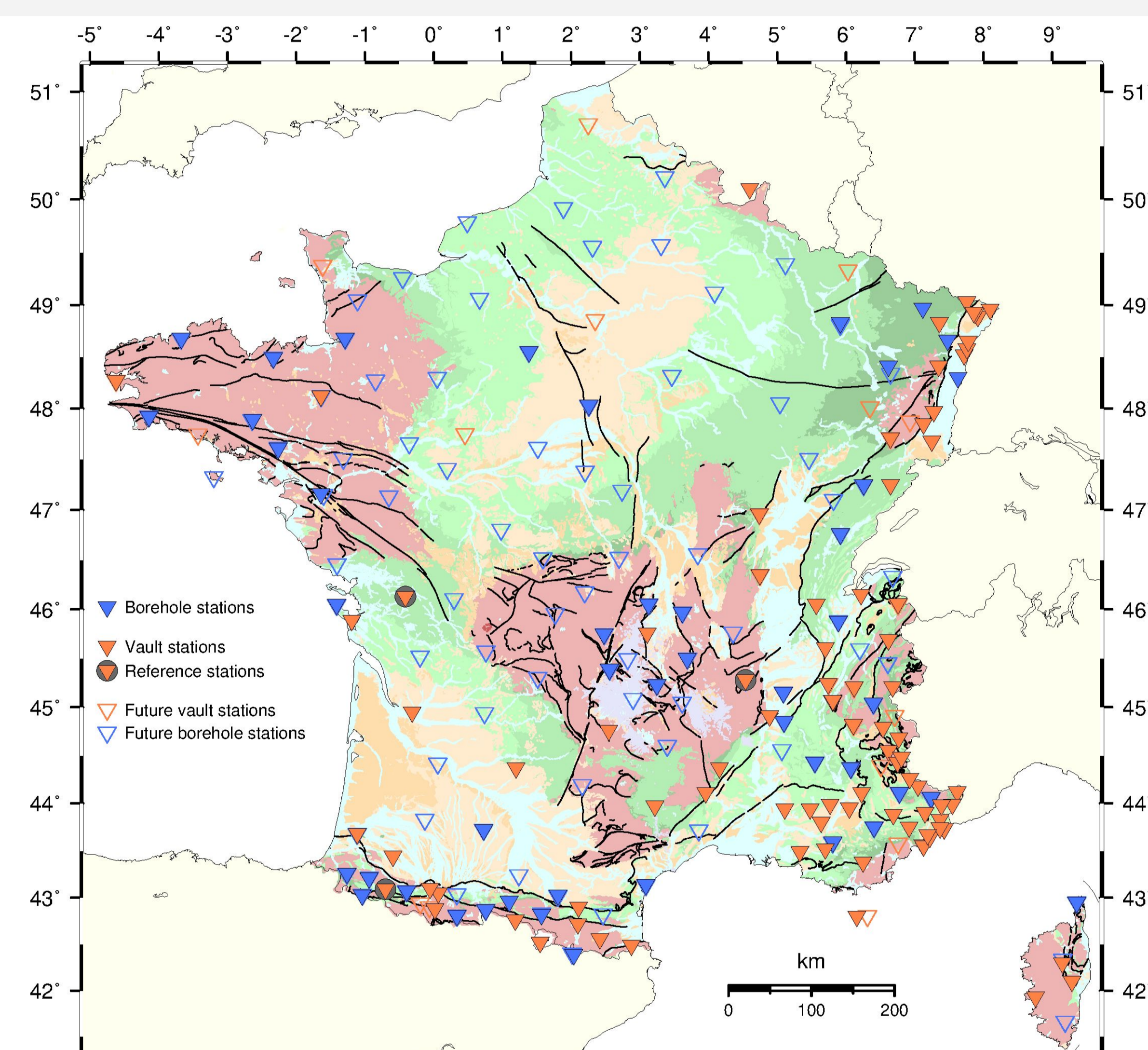
Figure 1.1 : Map of the RLBP network above the geologic map of France. Solid triangles represent the operating stations (used in the present study). Open triangles represent stations that will be installed by the end of 2020. Borehole stations are plotted in blue while "classical vault" installation are plotted in orange. Geology map legend is presented to the left.
