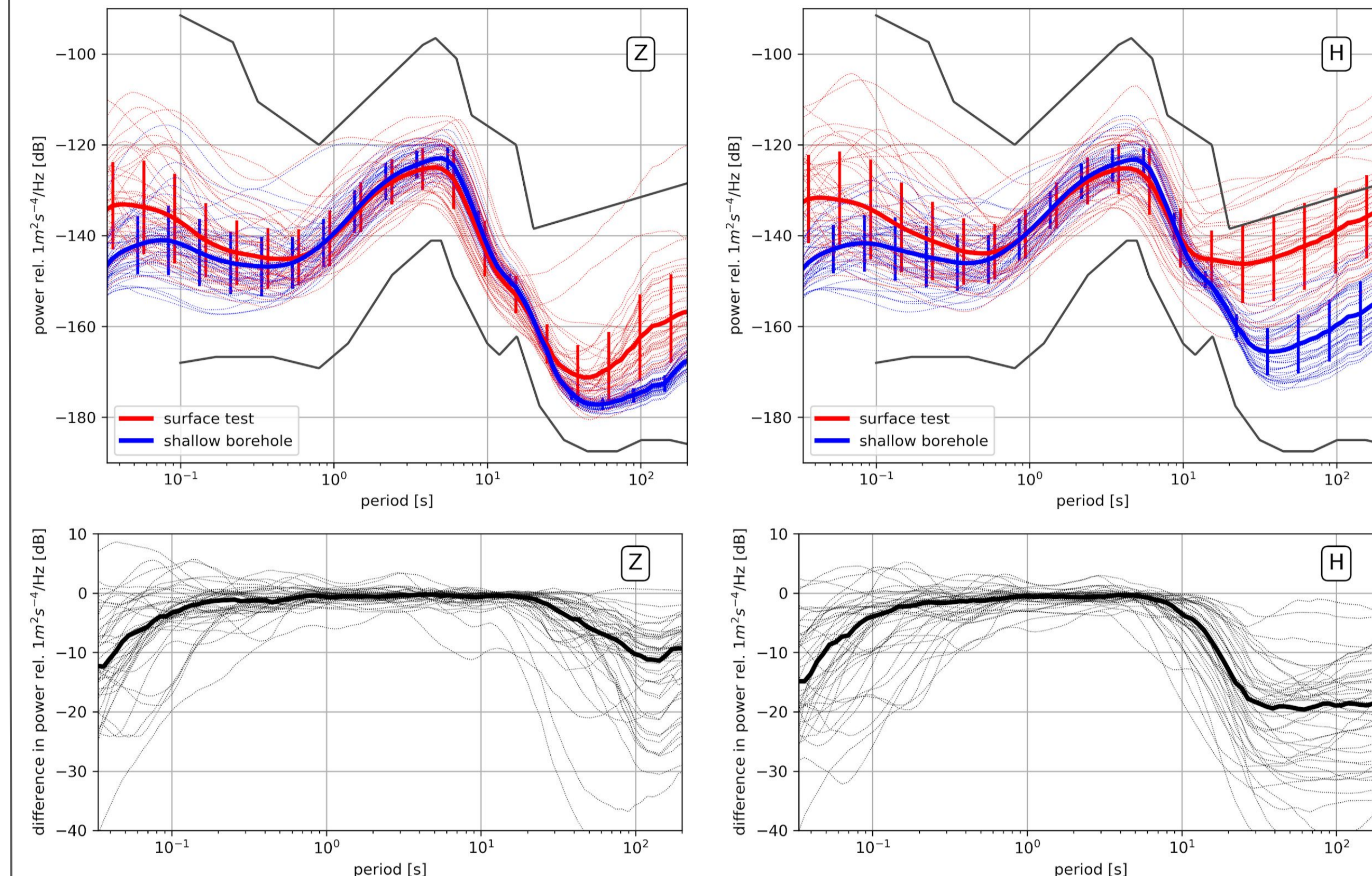
Figure 2.1 : (top) Median of the probability density function of the power spectral density functions (mPDF-PSD) of continuous records (dotted lines), following McNamara and Bulland (2004), for each of the 43 sites during their testing period (red) and in their final shallow borehole configuration (blue) for the vertical component (left) and the mean of the two horizontal components (right). Thick curves indicate the mean and standard deviation of the 43 mPDF-PSD for each configuration. (bottom) Difference between the test and shallow borehole mPDF-PSD for each site (dotted black lines) after correcting from the mPDF-PSD difference of a reference station (SSB, MLS, ATE or CHIF - see Fig. 1.1) computed for the two corresponding measuring periods. Thick thick lines correspond to the median of the individual differences. Note that the vertical scale goes from -40dB to +10dB.
