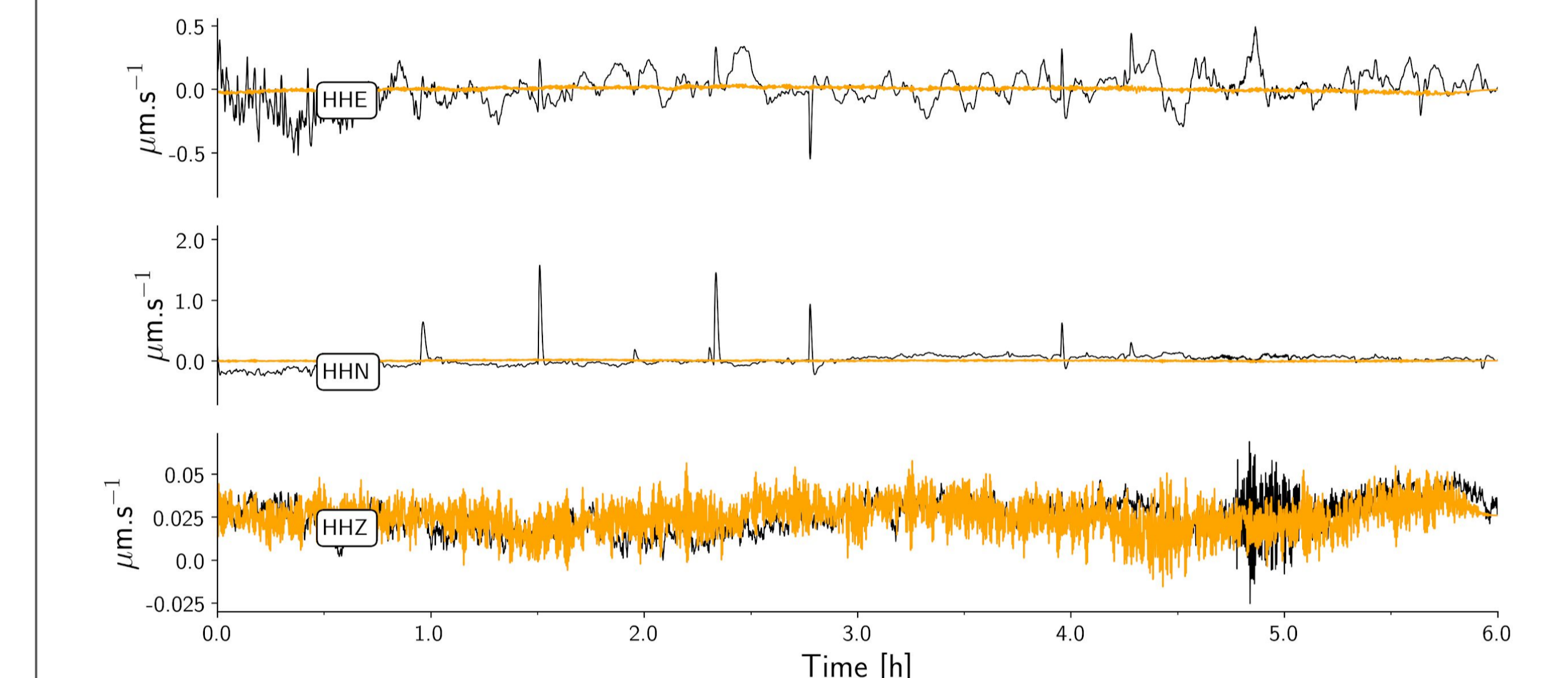
Figure 4.2 : 6 hours of filtered (lowpass at 1/20 Hz) traces at station BOUF. Solid black curves correspond to a period with no sand around the sensor and with cable issues (glitches). Solid orange curves correspond to a "well" installed sensor/cable with sand. The glitches are not detectable on the unfiltered traces but dramatically affect the noise level observed on PSD. Adding sand around the sensor has a dramatic effect of the noise level of the horizontal components at long period.
