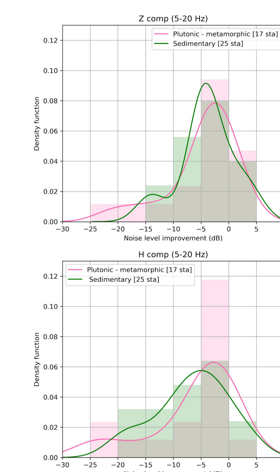
Figure 2.4 : Distribution of the mean difference in decibels of mPDF-PSD between the test and shallow borehole in the 5-20 Hz frequency range.
