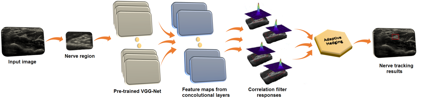
Fig. 2: Illustration of HDT tracker [40].
