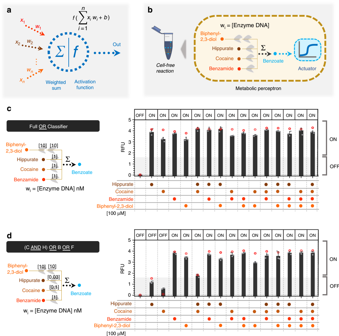
Fig. 6 Cell-free perceptron enabling development of classifiers. a A perceptron scheme showing the inputs and their associated weights, the computation core, and the output. The perceptron computes the weights and actuates the weighted sum through an activation function. b Metabolic perceptron integrating multiple inputs and actuating an output. The benzoate actuator acts as the activation function of the perceptron reporting the sum of benzoate produced by the metabolic perceptron. Hippurate, cocaine, benzamide, and biphenyl-2,3-diol are the inputs of the metabolic perceptron fixed to 100 \mu M. The weights of the perceptron are the concentration of the enzymes calculated using the model made on weighted metabolic circuits (red circles). These weights are calculated to develop two classifiers using the metabolic perceptron and benzoate actuator. Full OR classifier c , [cocaine (C) AND hippurate (H)] OR benzamide (B) OR biphenyl-2,3-diol (F) classifier d are the two classifiers built using this metabolic perceptron. The Full OR classifier ( c ) classifies to OFF when none of the inputs is present and it passes an arbitrary threshold to ON when any of the inputs or their combinations are present. The second classifier ( d ) performs a more complex computation. The shading represents the arbitrary threshold that allows for perceptron decision making and the panel of OFF and ON at the top of the bars are the expected output of the classifiers. All data are the mean and the error bars are the standard deviation of normalized values from three measurements and red circles are the model predictions (gray dots on each bar are individual values from which the mean and SD were calculated). (RFU relative fluorescence unit). Source data are provided in the Source Data file
