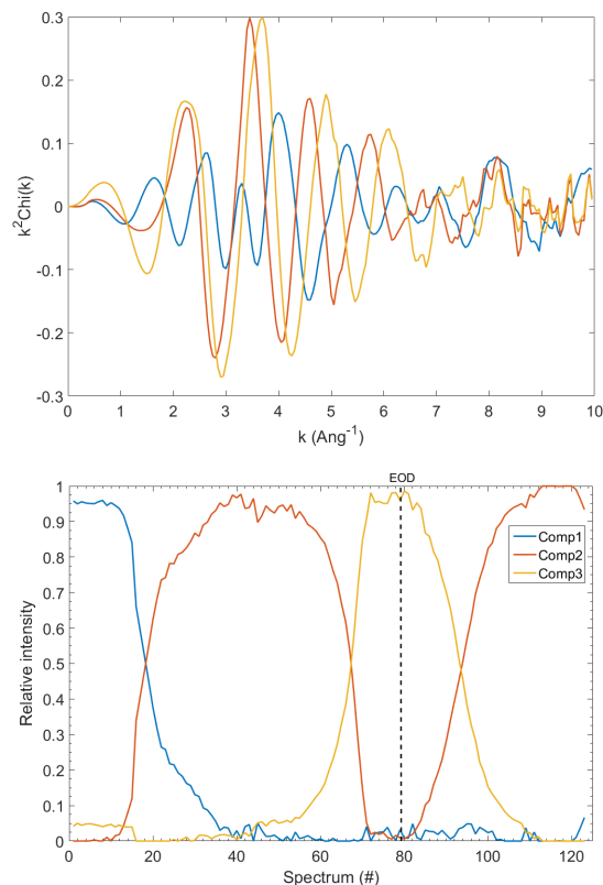
Figure 10: EXAFS spectral components (top) obtained by MCR-ALS analysis of the operando Bi L 3 -edge XAS spectra, and variation of their intensity (b) during electrochemical cycling. The vertical black line represent the end of the first discharge (EOD).
