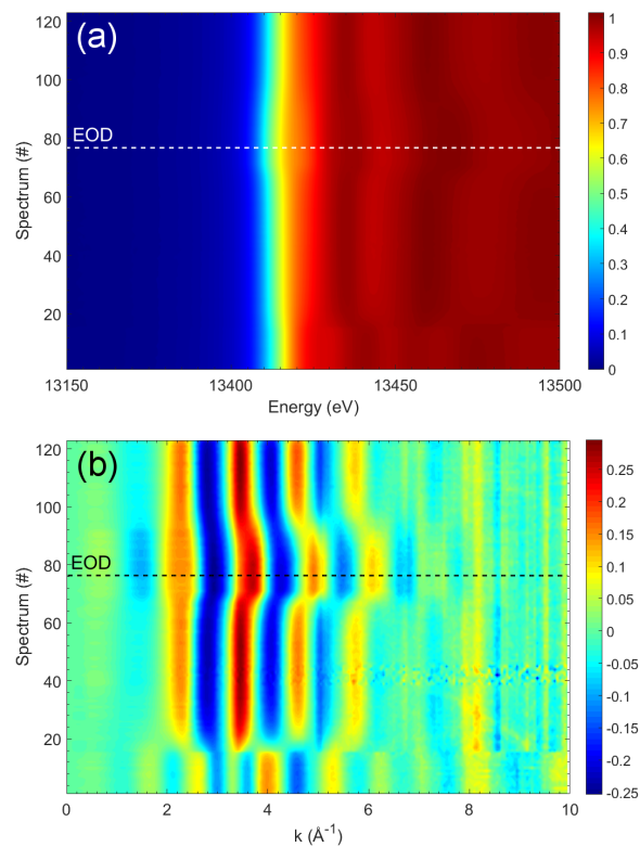
Figure 9: (a) XANES and (b) EXAFS operando Bi L 3 -edge XAS spectra measured during the first electrochemical cycles of BiSb electrode vs. Na. The horizontal line labelled EOD represents the end of the first discharge.
