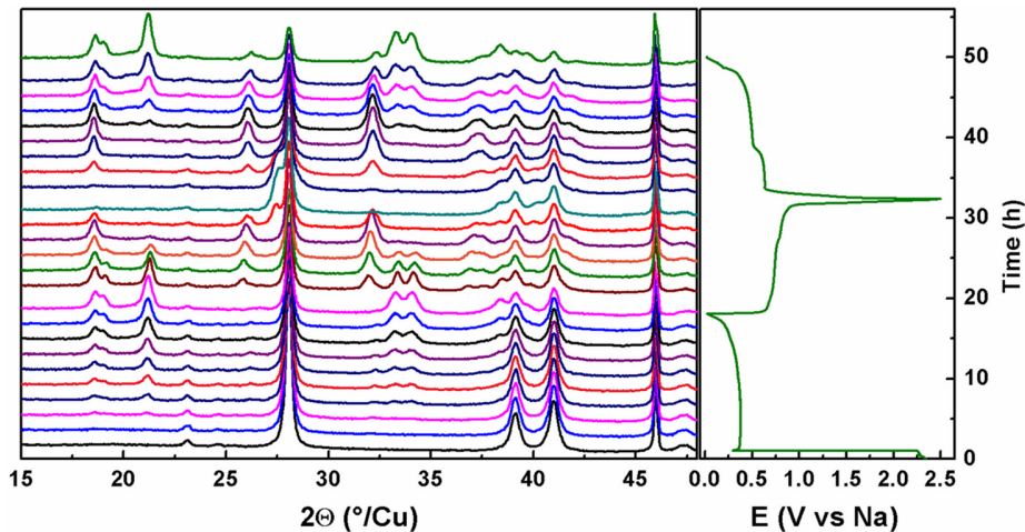
Figure 8: Operando XRD patterns collected at various stages of discharge and charge of BiSb (left) and the corresponding voltage profile (right).
