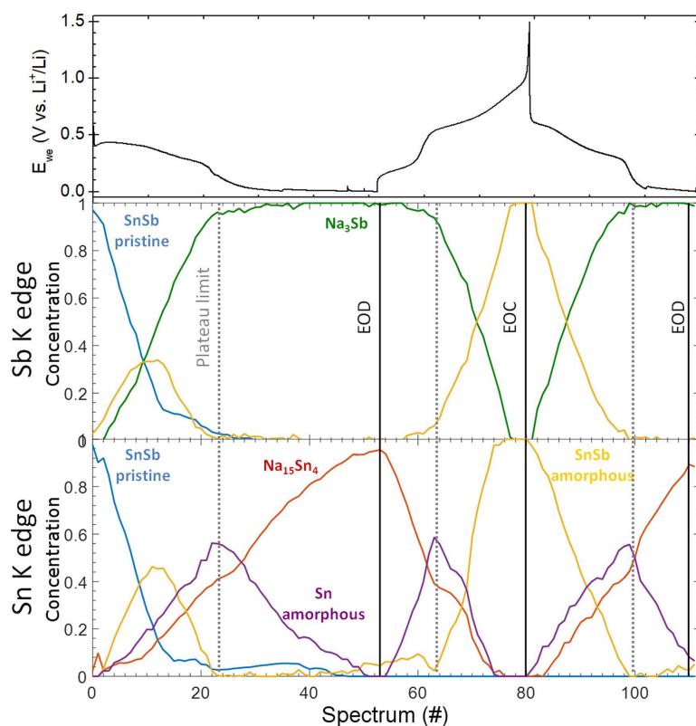
Figure 5: Evolution of the concentration of the MCR-ALS spectral components for Sn and Sb K-edges during subsequent sodiation, desodiation and sodiation of SnSb, and corresponding experimental electrochemical signature. EOD and EOC mean the end of discharge and end of charge, respectively.
