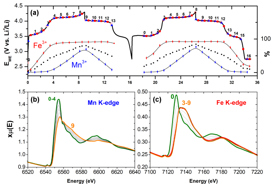
Figure 1: (a) Quantitative evaluation (in % of each metal) of the Fe 3+ and Mn 3+ content during the first two charge/discharge cycles obtained from the linear combination fitting of the operando Mn (b) and Fe (c) K-edge XANES spectra of LiFe 0.33 Mn 0.67 PO 4 recorded upon cell operation at C/10 rate (a). Some spectra between the two cycles could not be recorded due to beam loss during cycling.
