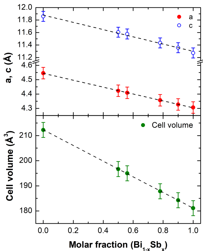
Figure 7: The variation of lattice parameters a and c (top) and that of the unit cell volume (bottom) versus the molar fraction x of antimony in \text{Bi}_{1-x}\text{Sb}_x alloys. The dashed lines should be considered as guides to the eye.
