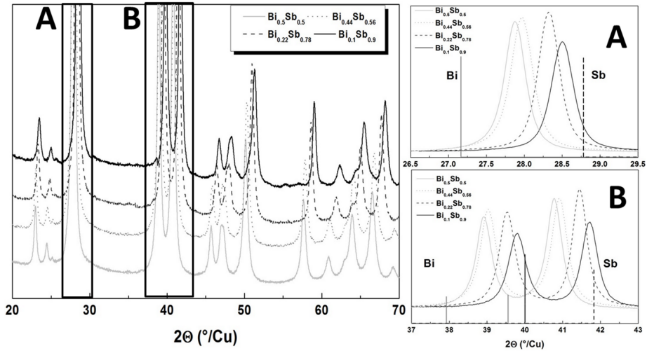
Figure 6: a) XRD patterns of \text{Bi}_{1-x}\text{Sb}_x alloys with x = 0.9, 0.78, 0.56, 0.5 (top to bottom); b) Evolution of the (012) diffraction profile for different concentrations of Sb; the position of the profiles of pure Sb and Bi (vertical lines) are presented for comparison.
