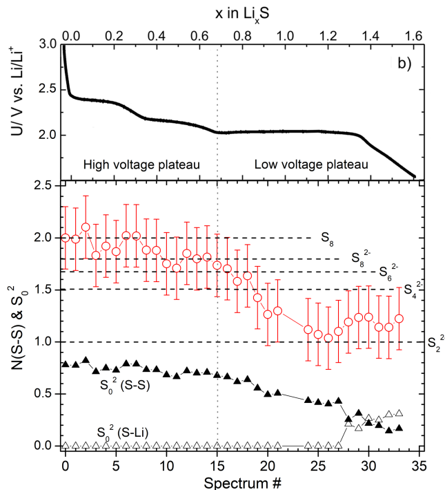
Figure 3: Average coordination number of S in sulfur and polysulfides (red circles) during the first discharge determined from the EXAFS spectra measured in the 1M LiTDI TEGDME:DOL electrolyte, and corresponding amplitude attenuation factor S_0^2 of the Li-S and S-S contributions, indicating the growth in intensity of \text{Li}_2\text{S} and the decrease of polysulfide contribution towards the end of the discharge. The average coordination of the most important polysulfides is represented by the horizontal dashed lines. The corresponding electrochemical curve measured during the discharge is shown on top.
