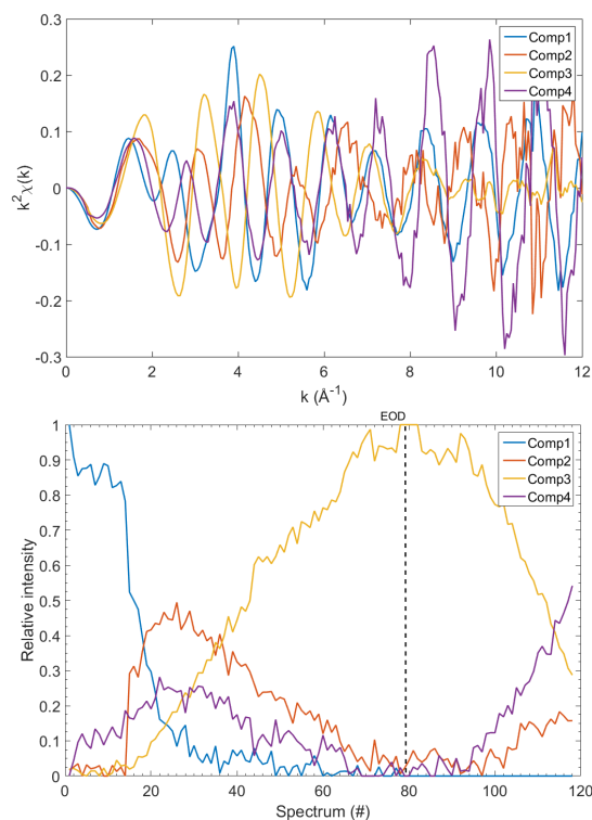
Figure 11: EXAFS spectral components (top) obtained by MCR-ALS analysis of the operando Sb K-edge XAS spectra, and variation of their intensity (b) during electrochemical cycling. The vertical black line represent the end of the first discharge (EOD).
