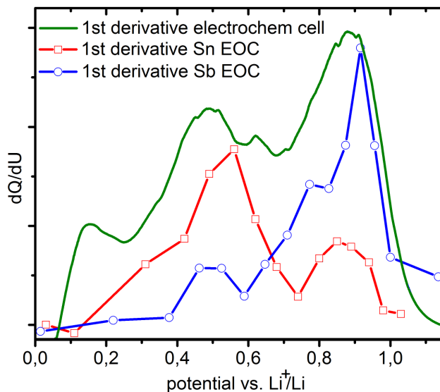
Figure 4: Derivatives of the MCR-ALS concentration profiles of the Sn (red) and Sb (blue) EOC components and overall dQ/dV profile measured in the operando cell (green) during charge.
