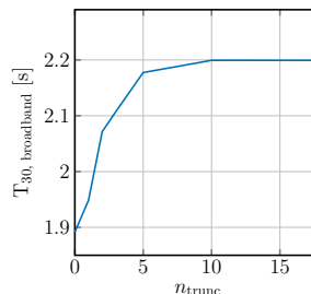
(c) T_{30,broadband} .
