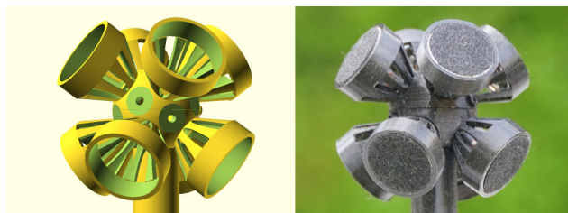
Figure 5. OctaSpHEAR v2 capsule array design
