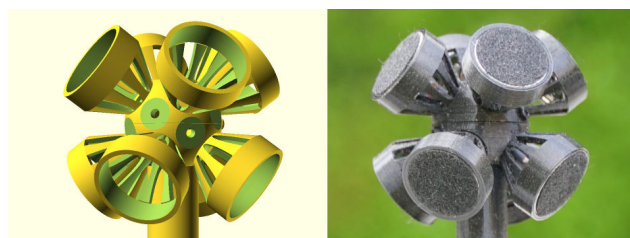
Figure 5. OctaSpHEAR v2 capsule array design
