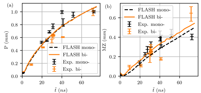
FIG. 4. Experimental interface position (a) and MZ (b) as a function of time, in both mono-mode and bi-mode cases, compared with the associated simulations. The time is rescaled by a factor of (E/E_0)^{1/3} to remove the variation in drive energy from shot to shot.
