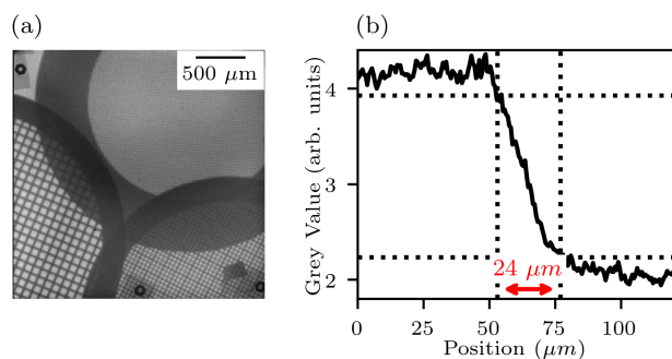
FIG. 2. (a): Radiograph of three gold grids (300, 600 and 1000 lines per inch) at target position. (b): Lineout of the border of a grid. A static resolution of 24 \mu\text{m} is measured (see red (light gray) arrow).
