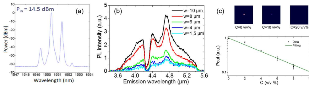
Fig. 2. a) Four-wave mixing spectrum obtained from 1-cm long selenides ridge waveguides, b) guided mid-IR photoluminescence spectrum from \text{Pr}^{3+} -doped selenides ridge waveguides c) Isopropanol detection @ 7.7 \mu\text{m} using selenides waveguides.
