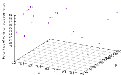
Fig. 2. Percentages of correctly segmented words using semi-supervised method with different values of \alpha and \beta
