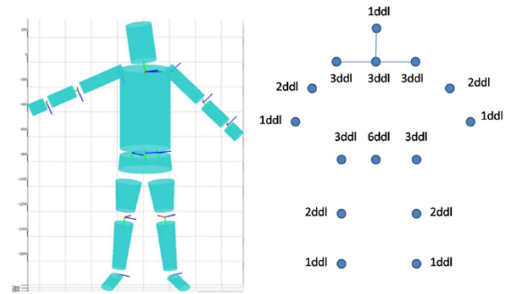
Figure 2: Degrees of freedom of the 3D model
