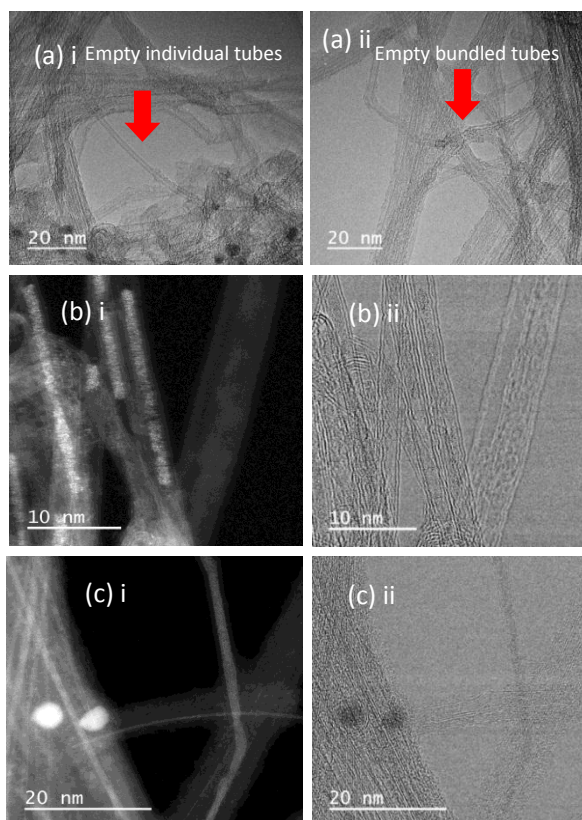
Fig 2: (a) (i and ii) HRTEM images of empty DWNTs showing individual and bundled DWNTs (b) STEM (i) High-angle annular dark field (HAADF) image of Zinc Acetate filled
