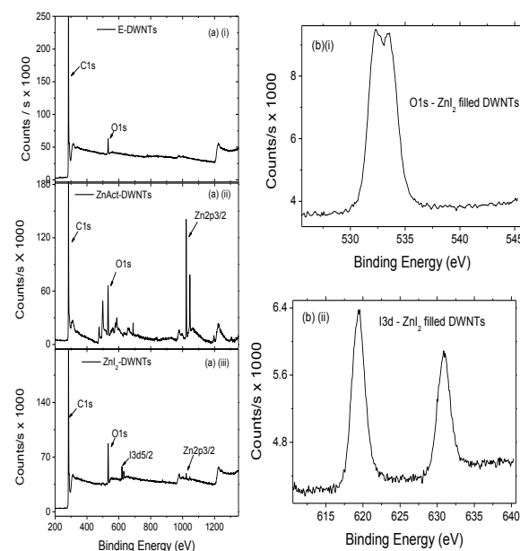
Fig 4: (a)(i) XPS survey spectra of raw DWNTs (ii) XPS survey spectra of Zinc acetate filled DWNTs (iii) XPS survey spectra of Zinc iodide filled DWNTs (b) (i) The O1s peaks of ZnI 2 filled DWNTs (ii) The I3d peaks for iodine filled DWNTs.
