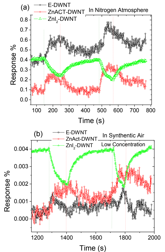
Fig 5: (a) Formaldehyde gas response of the three kinds of DWNTs measured in nitrogen atmosphere. (b) Formaldehyde gas response of the three kinds of DWNTs measured in synthetic air atmosphere. In both cases, during the first cycle the vapour mass concentration was 1.8 % as calculated using equation 1 and this was increased to 2.2 % during the second cycle by increasing the flow rate of the carrier gas. The olive green dotted vertical lines show when the respective vapour was introduced and the red lines indicate when the vapour was closed.
