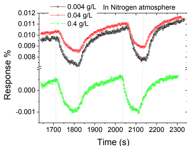
Fig 9: Response of Zinc Iodide filled DWNTs to 2.8 % (as calculated using equation 1) of formaldehyde diluted at different concentrations in deionised water. The second cycle is when vapour concentration was increased by 0.4 % by increasing the flow rate of the carrier gas. The olive green dotted vertical lines show when the respective vapour was introduced and the red lines indicate when the vapour was closed.
