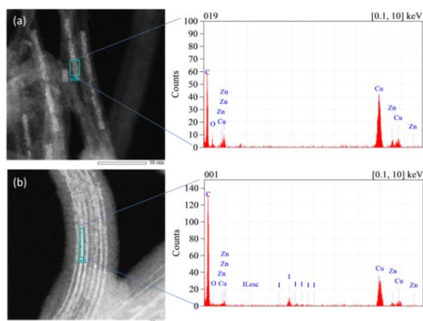
Fig 3: HAADF-STEM image and EDX analysis of the filled DWNTs (a) Zinc acetate filled DWNTs (b) Zinc iodide filled DWNTs.
