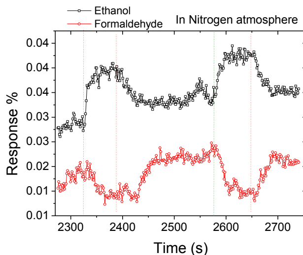
Fig 7: Response of iodine (only) - incorporated DWNTs to 2.8 % mass concentration of ethanol or 3.2 % of formaldehyde in nitrogen atmosphere (as calculated using equation 1). The second cycle is when vapour concentration was increased by 0.4 % by increasing the flow rate of the carrier gas. The olive green dotted vertical lines show when the respective vapour was introduced and the red lines indicate when the vapour was closed.
