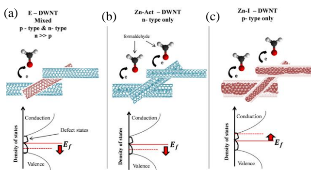
Fig 6: Schematic of the sensing mechanism as envisioned for different DWNTs samples under investigation. An approaching formaldehyde molecule will draw electrons from the DWNTs; this will push the Fermi level ( E_f ) down when the n-type DWNTs dominate the conduction (a and b) or push the Fermi level up when p-type DWNTs dominate (c).
