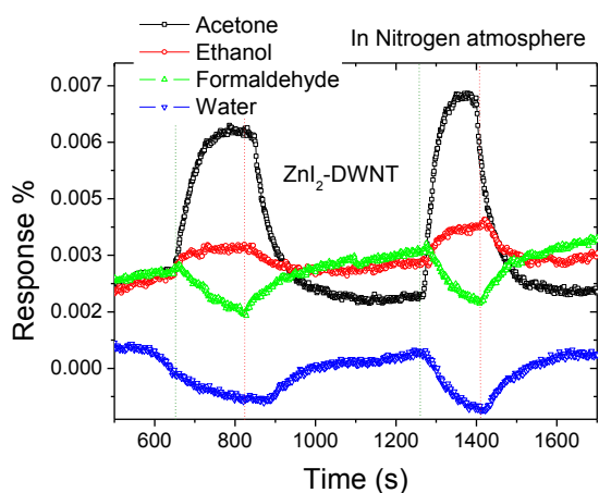
Fig 8: Response of Zinc Iodide filled DWNTs to different common volatile organic compounds (Acetone – 2.3%, Ethanol – 2.1%, Water – 2.0% and Formaldehyde – 2.8% as calculated using equation) in nitrogen atmosphere. The second cycle is when vapour concentration was increased by 0.4 % by increasing the flow rate of the carrier gas. The olive green dotted vertical lines show when the respective vapour was introduced and the red lines indicate when the vapour was closed.
