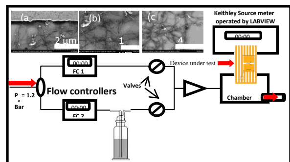
Fig 1: Illustration of the gas sensing system with LABVIEW software used for controlling the Keithley source meter and recording the data. Inset, a,b and c, typical SEM micrographs of sensing area of the device showing (a) the connection of DWNT networks to the gold electrode and (b, and c) entangled DWNTs between electrodes at different magnifications.
