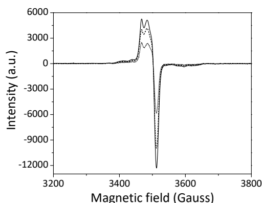
Figure 2. EPR spectra of electron-beam irradiated 9 \mu\text{m} thickness PVDF films at different doses: 5 kGy (dotted line), 7.5 kGy (dashed line), 10 kGy (solid line). Calculated g-value equals to 2.008 for central field of 3502.7 Gauss.
