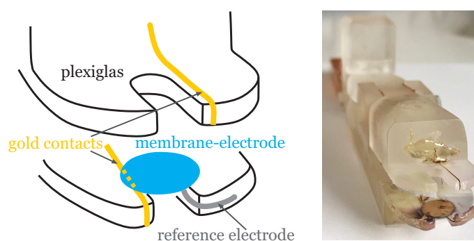
Figure 10. (a) Scheme of the clip set-up used for voltammetric measurements. (b) Photo of the clip with membrane electrode placed inside.
