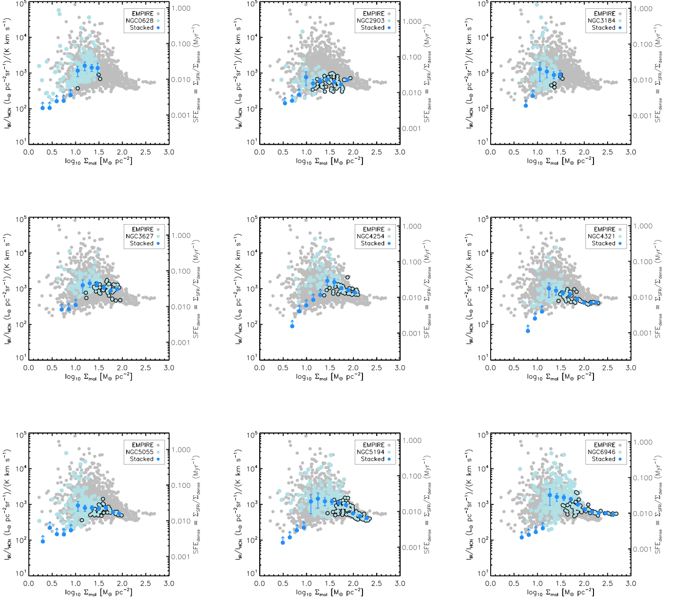
FIG. D6.— IR-to-HCN ratio (left axis) and \Sigma_{\text{SFR}}/\Sigma_{\text{HCN}} (right axis), tracing the efficiency of dense gas, as a function of density of molecular gas as traced by CO. The description of each data point is the same as in Figure D1. The dense gas efficiency appears to decrease for higher values of I_{\text{CO}} . We emphasize that NGC 2903 lacks Herschel data, and its SFR is calculated only using the available 24\mu\text{m} , which is a less accurate procedure.
