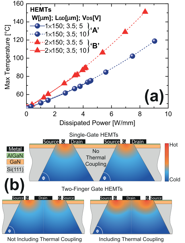
FIGURE 11. (a) Evolution of the maximum channel temperature versus the dissipated power density of single and two-finger gate AlGaIn/GaN HEMTs ('A': W = 1 \times 150\ \mu\text{m} ; and 'B': W = 2 \times 150\ \mu\text{m} ). The device dimensions are: L_{SG} = 1.0\ \mu\text{m} , L_G = 0.5\ \mu\text{m} , L_{GD} = 3.5\ \mu\text{m} . (b) Illustration of the heat spreading angle in single and two-finger gate AlGaIn/GaN HEMTs.
