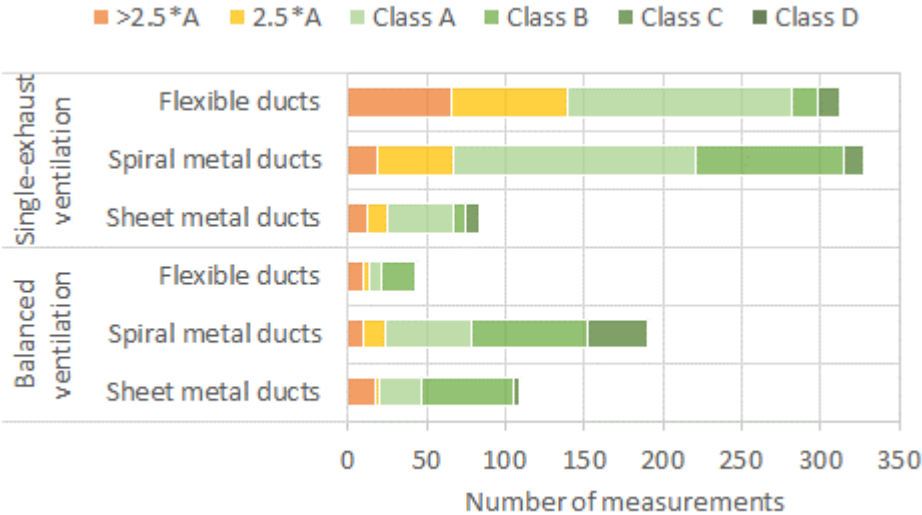
Figure 8: Distribution of ductwork airtightness measured classes depending on type of ventilation systems and implemented ducts
