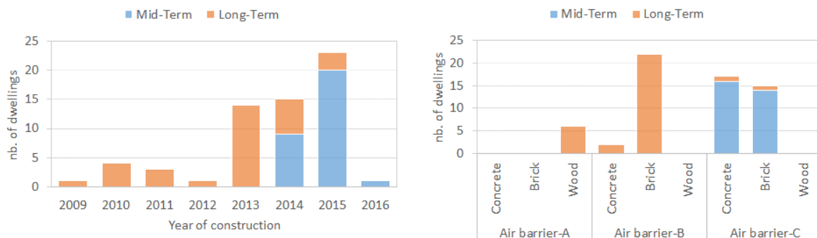
Figure 1: Distribution of buildings depending on the year of construction (left) and buildings main material and type of air barrier (right); Air barrier-A when the air barrier is ensured by vapour barrier, Air barrier-B by coating on the masonry, and Air barrier C by plasterboards and mastics at the inside facing of the walls
